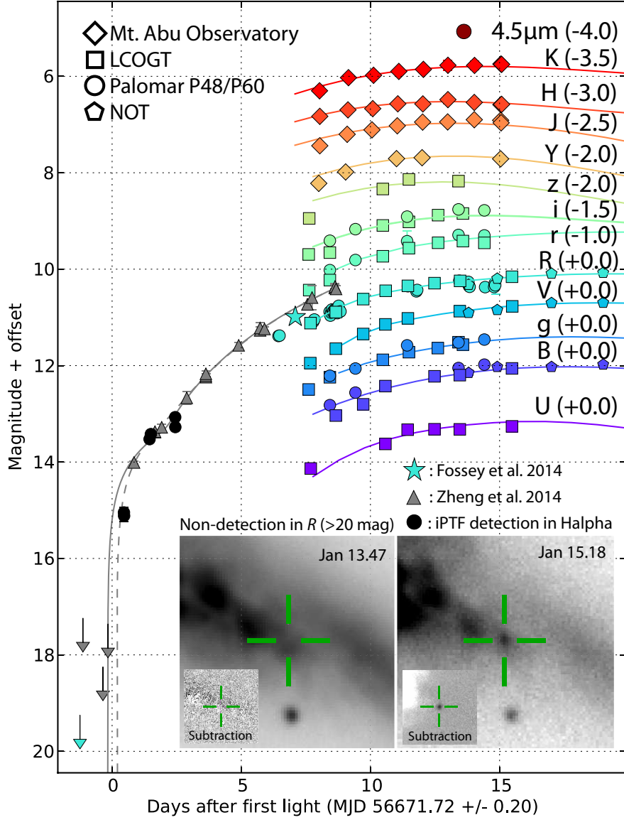
Fig. 2.— Lightcurves showing the rise of SN 2014J, along with SNOOpy fits described in the text. The first P48 H_\alpha^{656} and H_\alpha^{663} narrow bands detections are shown (black circles and inset image), S-corrected (Stritzinger et al. 2002) to R -band. Due to lack of accurate absolute calibration for the H_\alpha filters, a common offset was applied to connect with the data-points in the pre-discovery light curve presented in Zheng et al. (2014). We also show their two fits of t_0 , suggesting our first detection could be within \sim 5 hours from the onset of the supernova.
