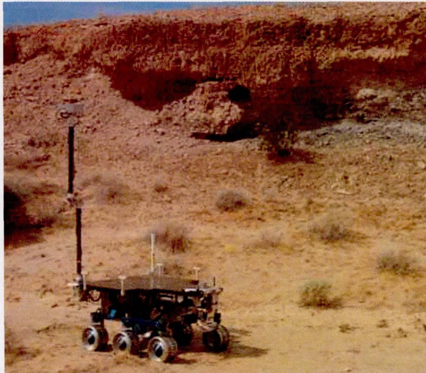
"FIDO" (Field-Integrated Design & Operations), a prototype Mars robotic explorer, being tested in the Mojave desert (picture courtesy NASA)
