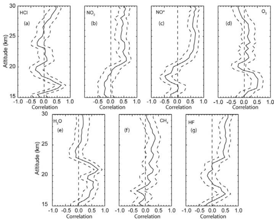
Fig. 11. Correlation of 5.26 \mu\text{m} anomalies based on the HALOE 3.46 \mu\text{m} model with HALOE measured species.
