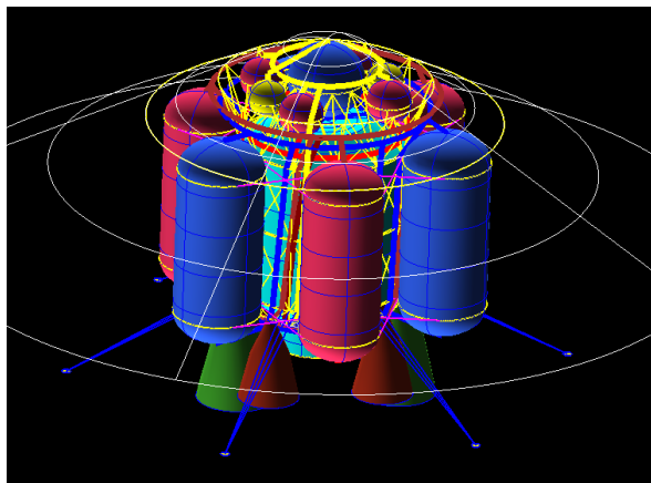
Figure 2—MAST I with lining shown
