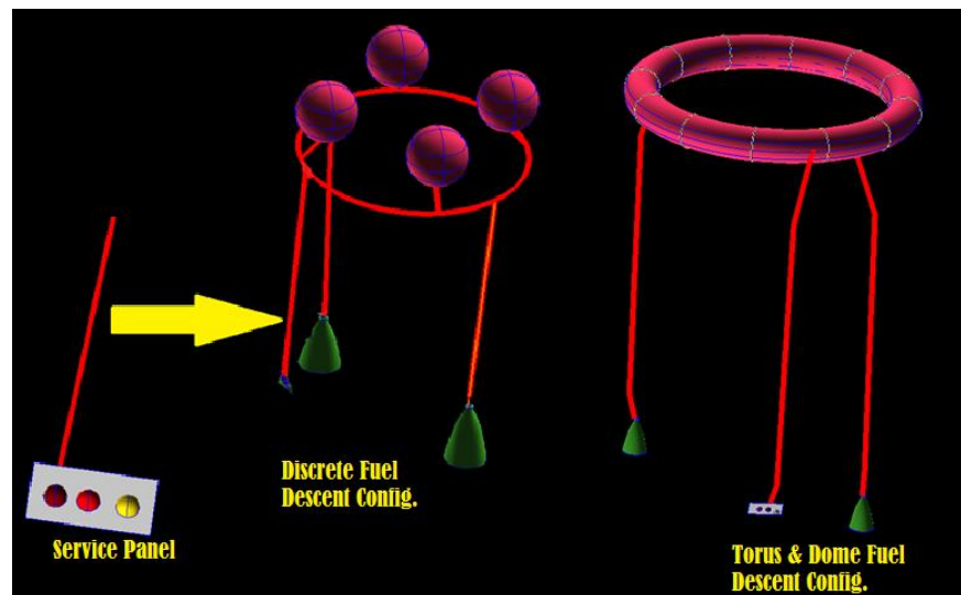
Figure 3--Example of fluid path configuration for fuel – between discrete and Torus/Dome
