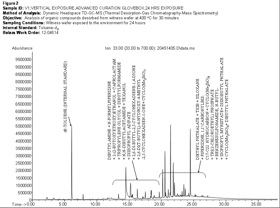
Figure 59: ACG Balazs organic wafer TD-GC-MS plot for vertical wafer exposure.
