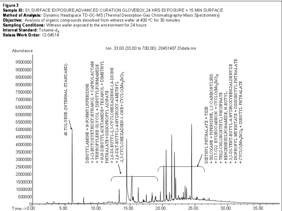
Figure 60: ACG Balazs organic wafer TD-GC-MS plot for surface wafer exposure.
