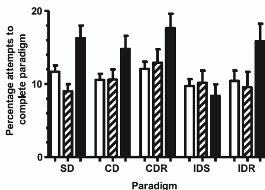
Figure 11. Effect of whole-body exposure to 1 GeV/nucleon ^{56}\text{Fe} particles on the paradigm-specific performance of retired breeder rats: number of attempts required to reach the criterion following sham-irradiation (open bar) and whole-body exposure to 15 cGy (hatched bar) or 20 cGy (solid bar) 1 GeV/nucleon ^{56}\text{Fe} . Graphs show means \pm SEM. HAB: habituation; SD: simple discrimination; CD: compound discrimination; CDR: compound discrimination reversal; IDS: intradimensional shifting; IDR: intra-dimensional shifting reversal; EDS: extra-dimensional shifting; EDR: extra-dimensional shifting reversal. Reproduced from Figure 5 of Britten et al. (2014).
