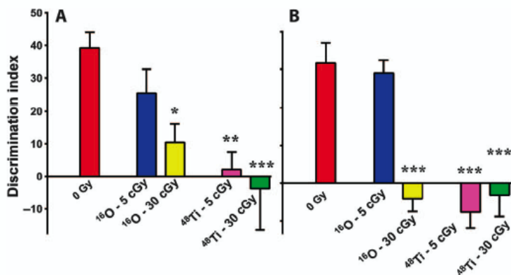
Figure 10. Behavioral deficits measured 6 weeks after charged particle exposure. (A) Performance on a NOR task reveals significant decrements in recognition memory indicated by the reduced discrimination of novelty. (B) Performance on an OiP task shows significant decrements in spatial memory retention, again indicated by a markedly reduced preference to explore novelty. * P = 0.05 , ** P = 0.01 , *** P = 0.001 , analysis of variance (ANOVA). Reproduced from Figure 1 of Parihar et al. (2015).
