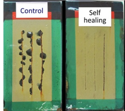
1000 hour salt fog testing result
