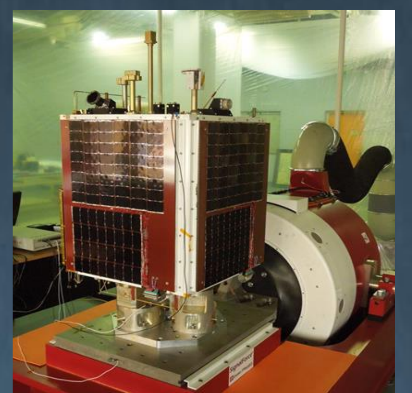
Figure 12. Saudi-Sat4 and UV-LED integrated, on shake table post random vibration
