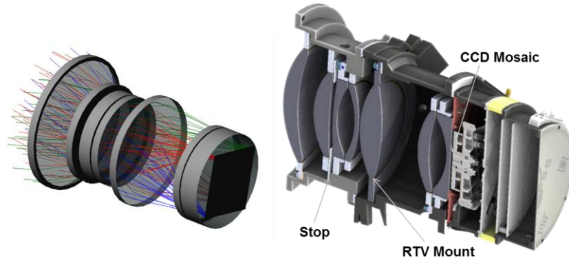
Figure 4 Lens Assembly
