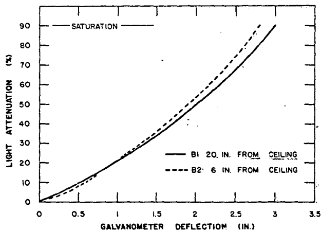
Figure 2. Smoke detector calibration curves, control aircraft.
