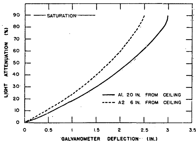
Figure 3. Smoke detector calibration curves, test aircraft.
