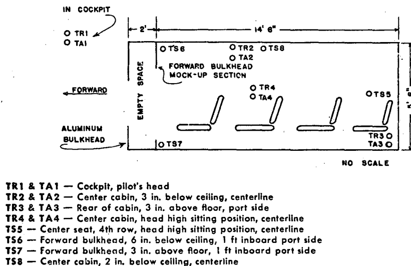
Figure 1. Thermocouple locations for Cleveland fire tests.
