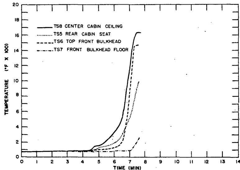
Figure 9. Temperature measurements in test aircraft, Test 2.
