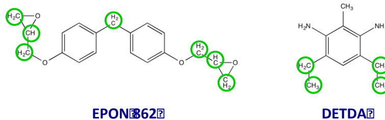
Figure 1: Molecular structures of EPON 862 and DETDA. Green atoms indicate united atoms.
