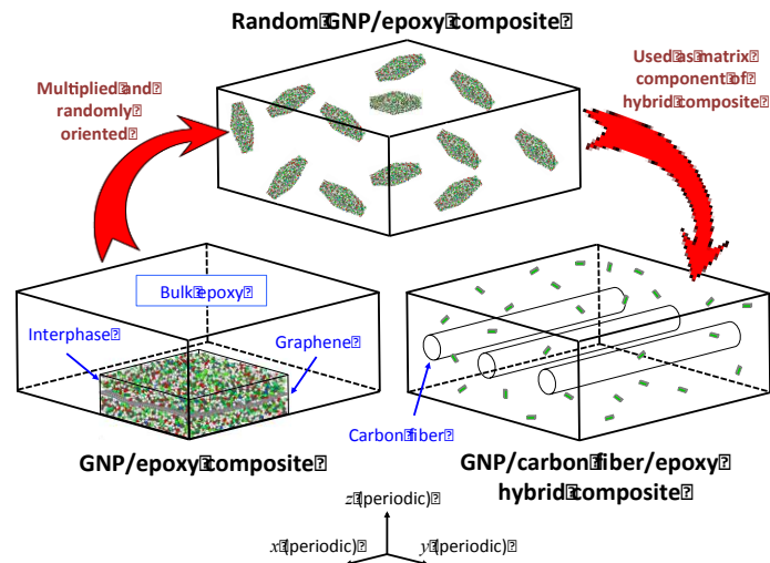
Figure 4: Multiscale modeling scheme.
