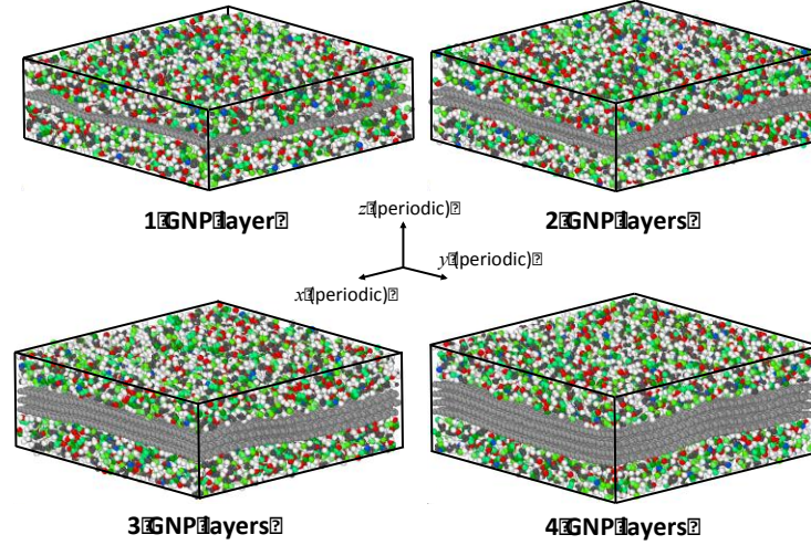
Figure 3: Equilibrated models for varying number of graphene layers.
