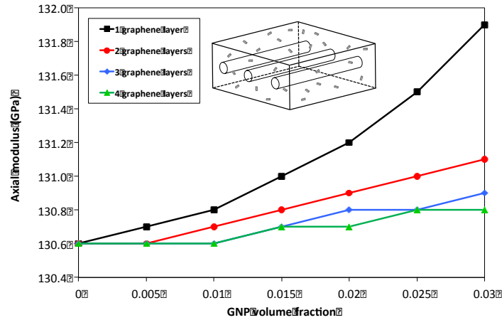
Figure 5: Predicted axial modulus for GNP/carbon fiber/epoxy hybrid composite.
