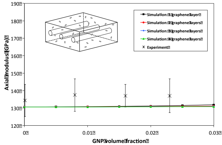
Figure 8: Axial modulus of GNP/carbon fiber/epoxy composite.
