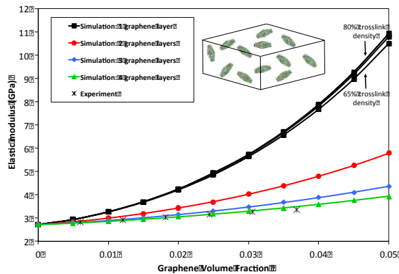
Figure 7: Modulus of GNP/epoxy composite for computational and experimental approaches.
