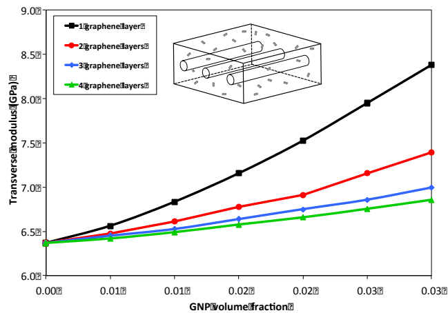
Figure 6: Predicted transverse modulus for GNP/carbon fiber/epoxy hybrid composite.
