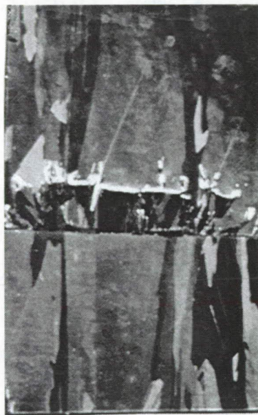
Figure 1. Photomicrograph showing the thermomigration of an aluminum zone through solid silicon.
