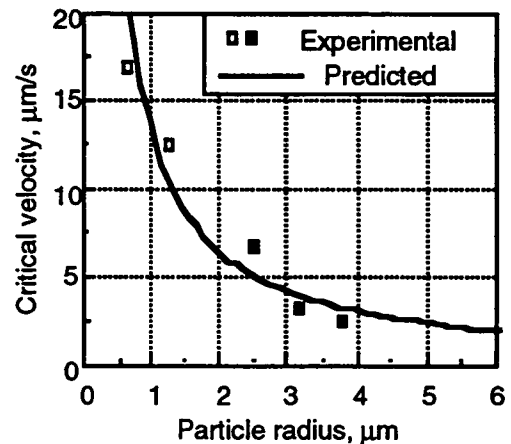
Fig. 2 Correlation between the critical velocity and particle radius in pure SCN ( G_L=108 \text{ K/cm} ).
