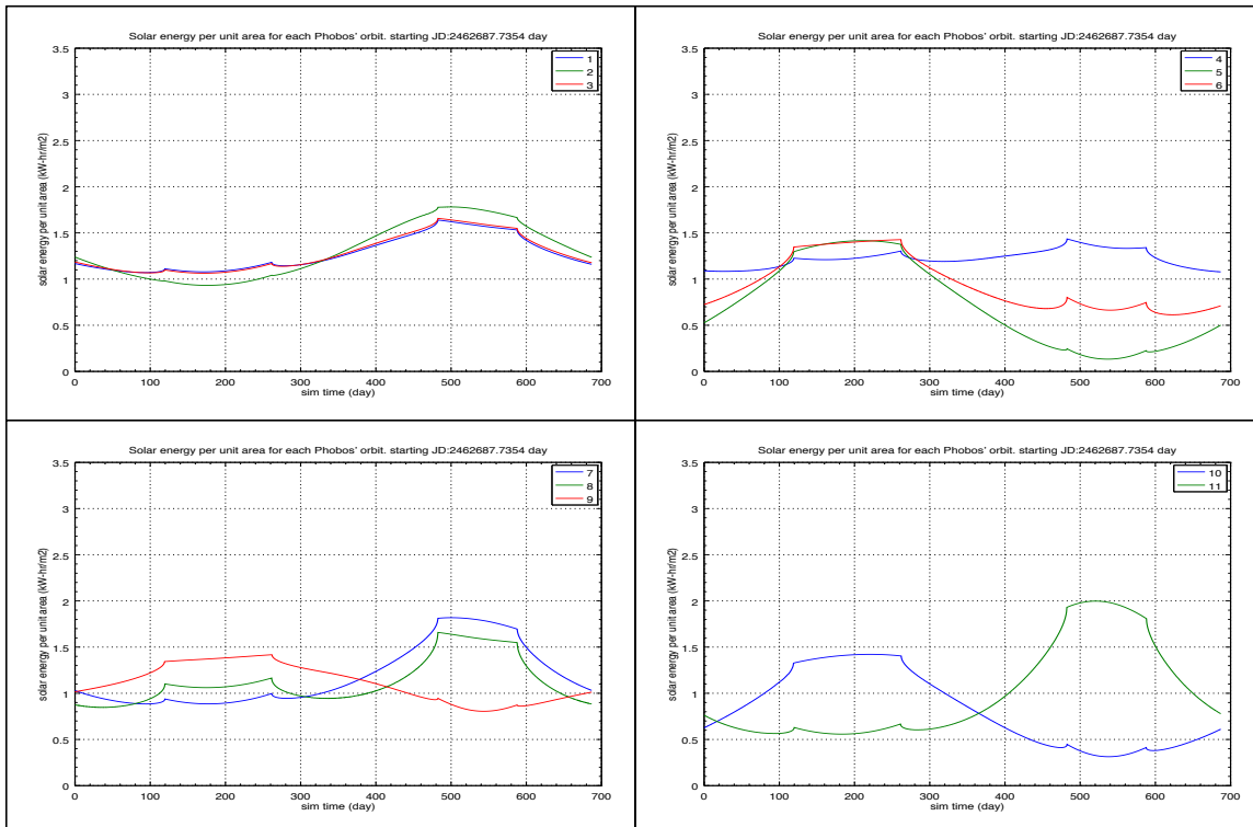
Figure 10. Energy per unit area per Phobos' orbit for a fixed array for site 1 to 11 ( kW \cdot hr/m^2 )
