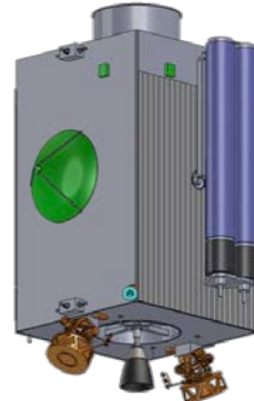
Figure 19. Concept for 25-kW hybrid solar-electric/chemical propulsion spacecraft for Mars mission (exterior view).
