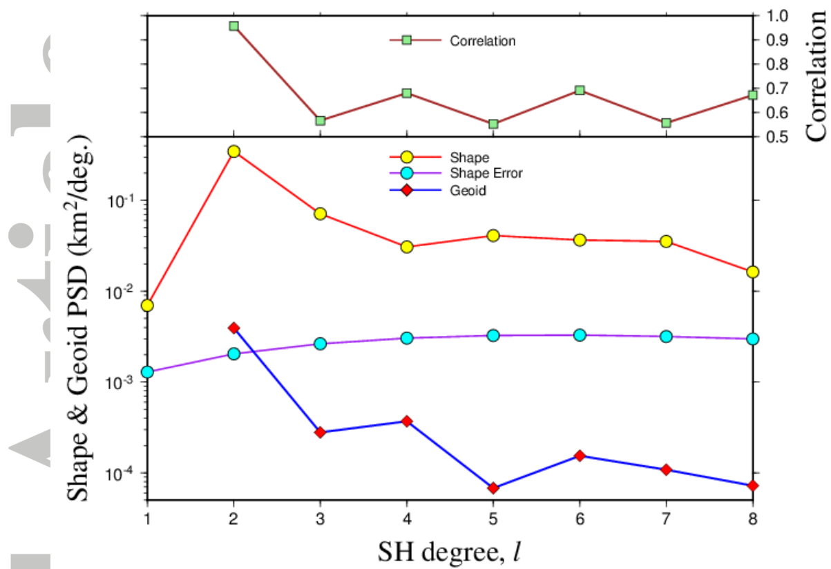
Figure 4. Power spectral density for Mercury's shape and geoid and the correlation between the two, which is particularly high at degree 2. The errors in the shape are lower bounds (see text).
