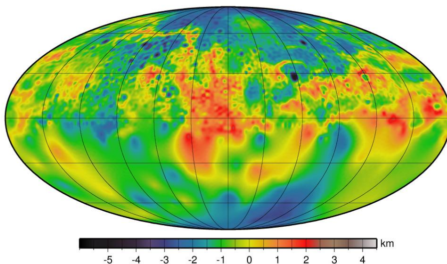
Figure 2. Shape of Mercury from a damped, spherical harmonic fit, to degree and order 128, to the MLA and occultation data shown in Figure 1. Color bar gives elevation in km.
