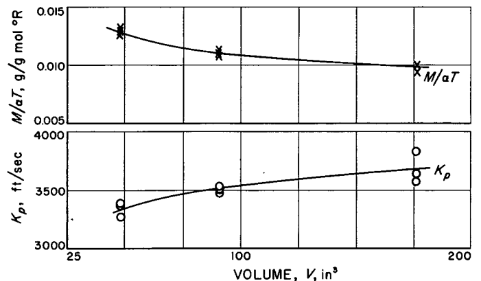
Figure 11. Plot of K_p and M/\alpha T vs chamber volume for cellulose acetate-lined chambers
