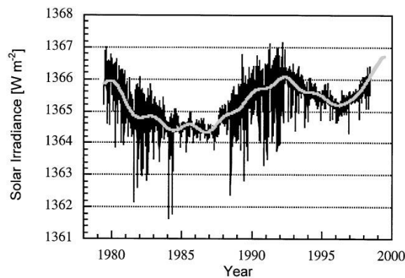
Figure 6. Measurement of Solar Irradiance.
