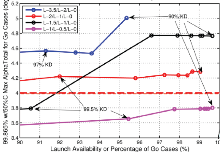
SLS DAC2-R Launch Availability Results
