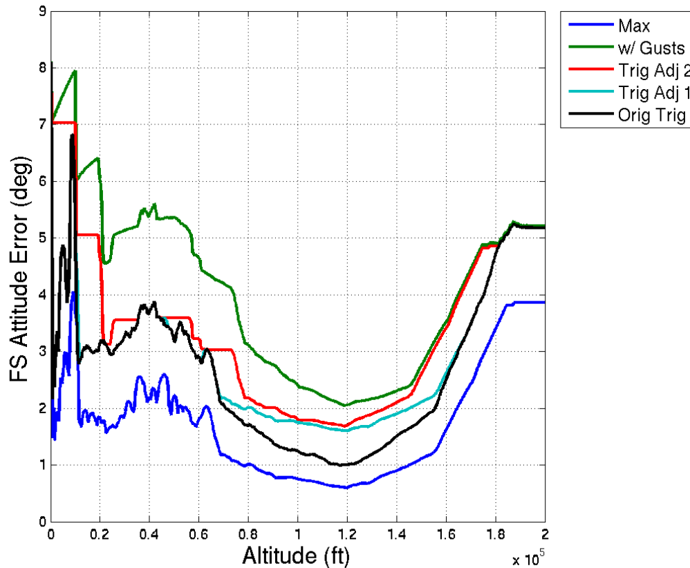
Abort Trigger Setting
