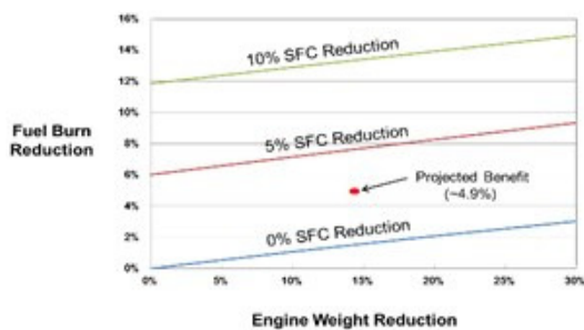
Figure 1: Regional jet fuel burn sensitivities showing reduction in fuel burn and engine weights.
