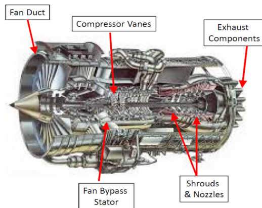
Figure 2: High-payoff engine components identified for advanced materials and manufacturing technologies.
