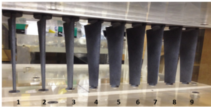
Figure 4: Inlet Guide Vane Cascade Test Section
