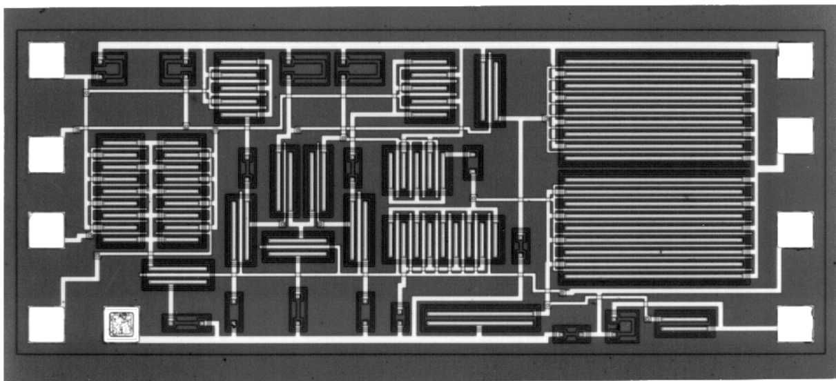
Figure 8. Optical micrograph of 1 \times 2 \text{ mm}^2 300 \text{ }^\circ\text{C} 6H-SiC operational amplifier integrated circuit. The chip contains 14 depletion-mode N-channel MOSFET's integrated with 19 resistors (From [105]. With permission)
