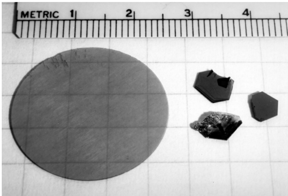
Figure 4. Mass-produced 2.5 cm diameter 6H-SiC wafer manufactured circa 1990 via seeded sublimation by Cree Research (left), and 6H-SiC Lely and Acheson platelet crystals (right) representative of single-crystal SiC substrates available prior to 1989. 5.1 cm diameter seeded sublimation SiC wafers entered the commercial market in 1997.
