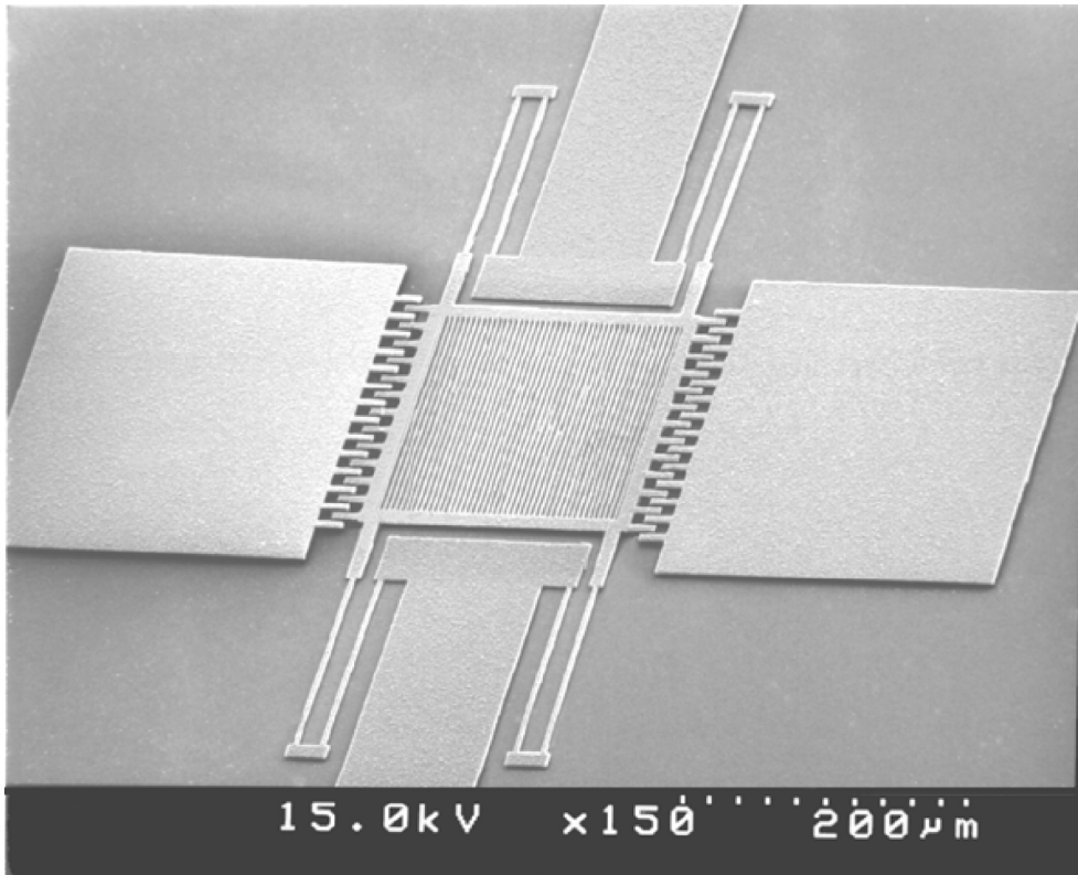
Figure 10. Micromachined SiC-based lateral resonator device. SiC's excellent mechanical and electrical properties are enabling the development of harsh-environment microelectromechanical systems (MEMS) for operation beyond the limits of conventional silicon-based MEMS. (From Prof. M. Mehregany, Case Western Reserve University. With permission.)
