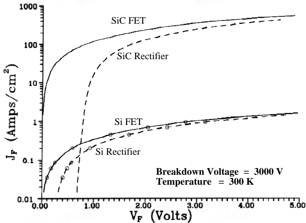
Figure 3. Simulated forward conduction characteristics of ideal Si and SiC 3000 V power MOSFET's and Schottky rectifiers. The high breakdown field of SiC relative to silicon (Table 1) enables the blocking voltage region (N-Drift Region in Figure 2) to be roughly 10X thinner and 10X heavier-doped, permitting a roughly 100-fold increase in on-state current density for the 3000 V SiC devices relative to 3000 V silicon devices. (From [8]. With permission.)
