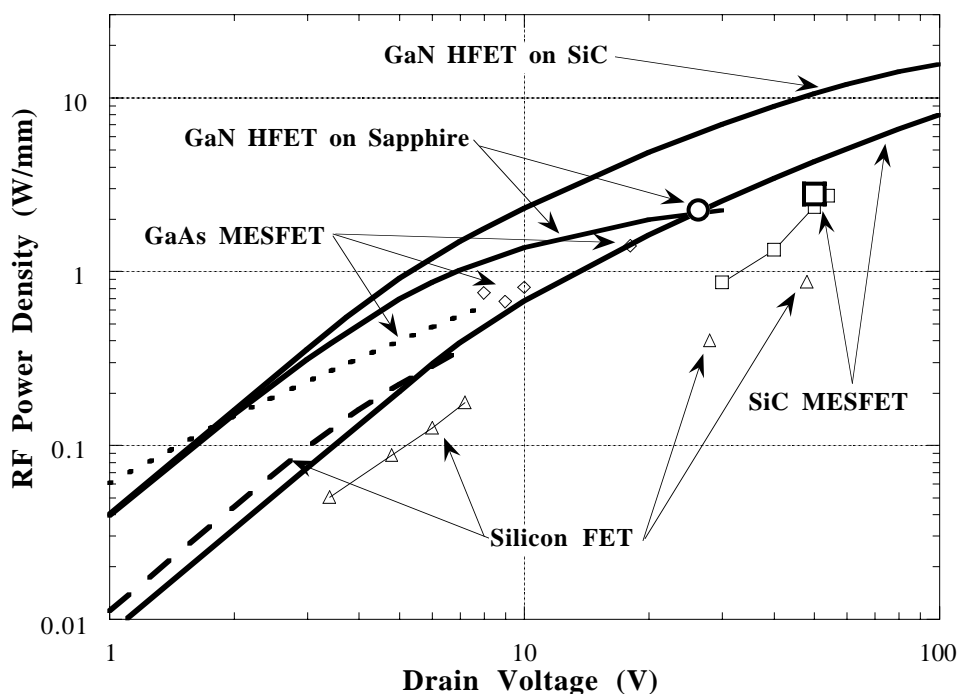
Figure 7. Theoretical (lines) and experimental (symbols) RF power densities of RF transistors fabricated in silicon, GaAs, SiC, and GaN as of late 1997. (From [96]. With permission.)
