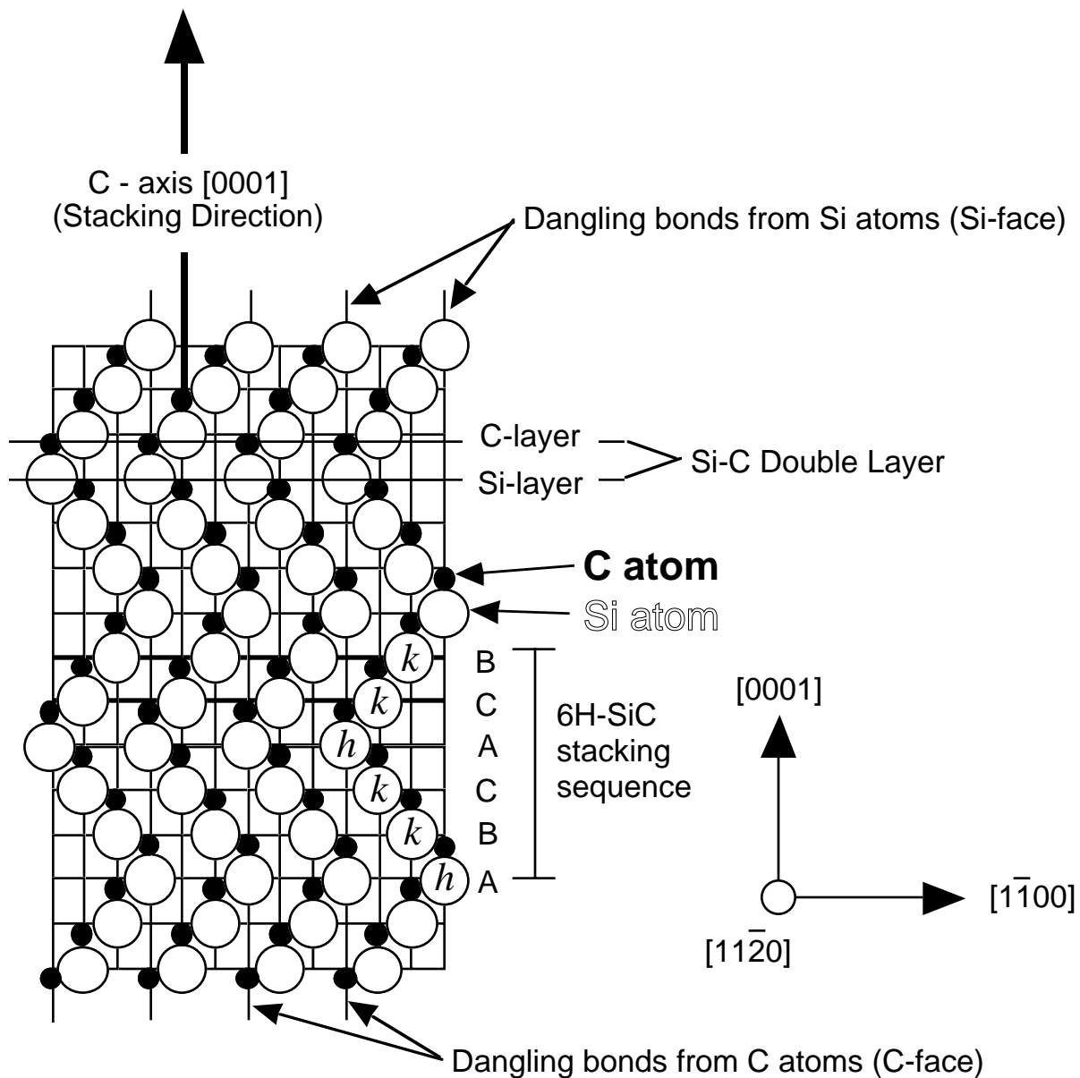
Figure 1. Schematic cross-section { (1120) plane } of the 6H-SiC polytype. (Modified from [10]. With permission)
