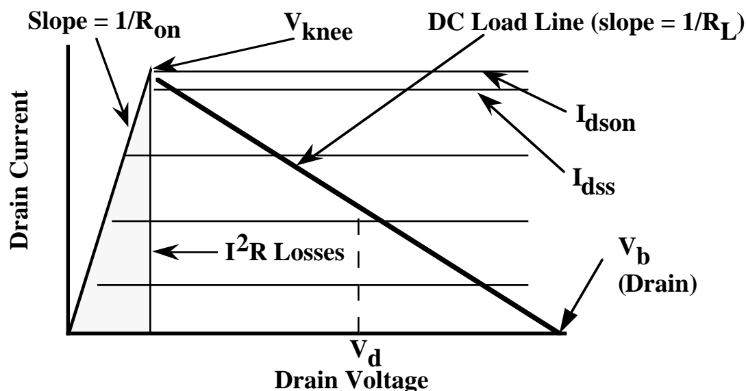
Figure 6. Piecewise linear MESFET drain characteristic showing DC load line used in Class A RF amplifier operation. The higher breakdown voltage V_b enabled by SiC's higher breakdown field enables operation at higher drain biases, leading to higher RF power densities. (From [7]. With permission.)
