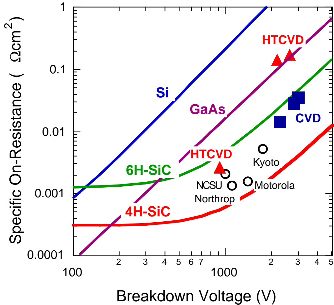
Figure 9. Experimental SiC (symbols) and theoretical SiC and silicon (lines) Schottky diode specific on resistance plotted as a function of off-state blocking voltage. While the graph clearly shows that the area-normalized performance of small-area SiC devices is orders of magnitude better than silicon, these results have not been successfully upscaled to realize large-area high-current SiC devices due to high densities of device-degrading defects present in commercial SiC wafers and epilayers. (From [117]. With permission.)
