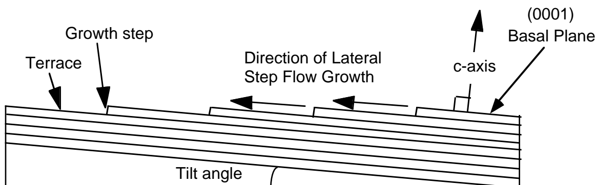
Figure 5. Cross-sectional schematic representation of “off-axis” polished SiC surface used for homoepitaxial growth. When growth conditions are properly controlled and there is a sufficiently short distance between steps, Si and C adatoms impinging onto the growth surface find their way to steps where they bond and incorporate into the crystal. Thus ordered lateral “step flow” growth takes place which enables the polytypic stacking sequence of the substrate to be exactly mirrored in the growing epilayer. (Modified from [10]. With permission)
