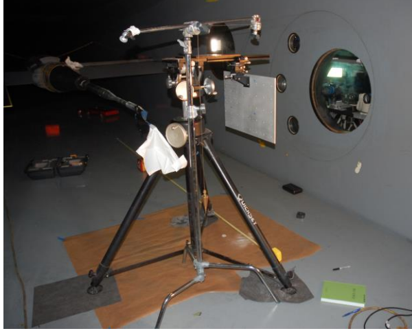
Figure 4. Calibration plate installed in test section. Figure 5. Applying speckles to Performance model.
