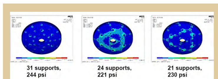
Fig. 4. Different support types demonstrated by mirror modeler.
