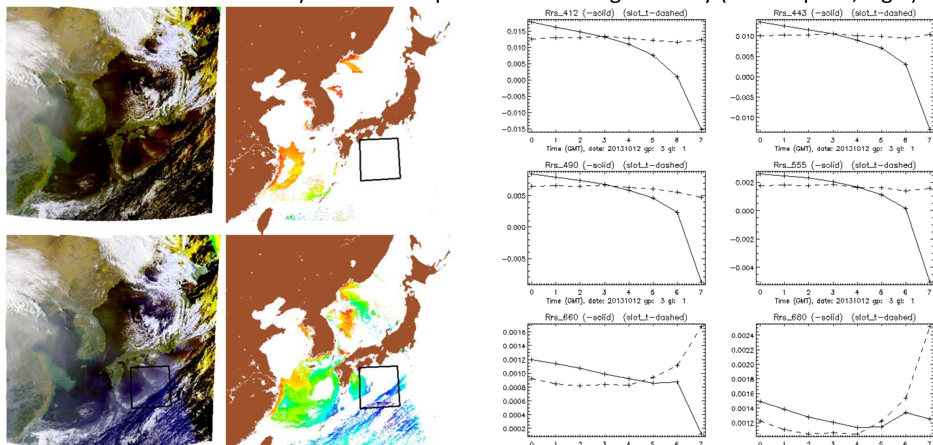
Figure 1. True color (left column) and chlorophyll-a (right column) for the 1600 local time GOCI scene on 12 Oct 2013. The top row was generated using one time for the entire scene while the bottom row uses the slot-based times. The 1600 time is affected the most by low solar zenith angles.
