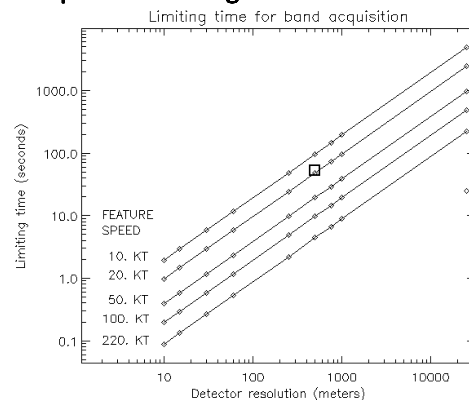
Figure 9. The maximum time allowed to acquire all bands for a pixel so that the feature, clouds in this case, will move by less than the detector size. GOCI is indicated by the square on the plot.
