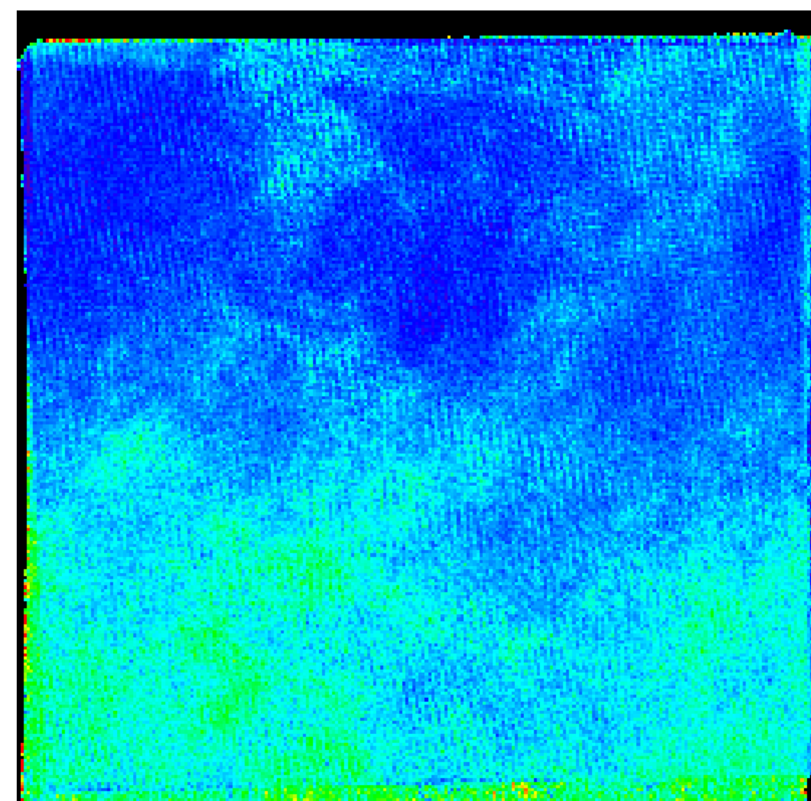
Figure 3. Image of 865 nm AOT slot-binned for 14 Aug 2012. The higher AOT (greens) consistently occur at the South end (bottom) of the slots.
