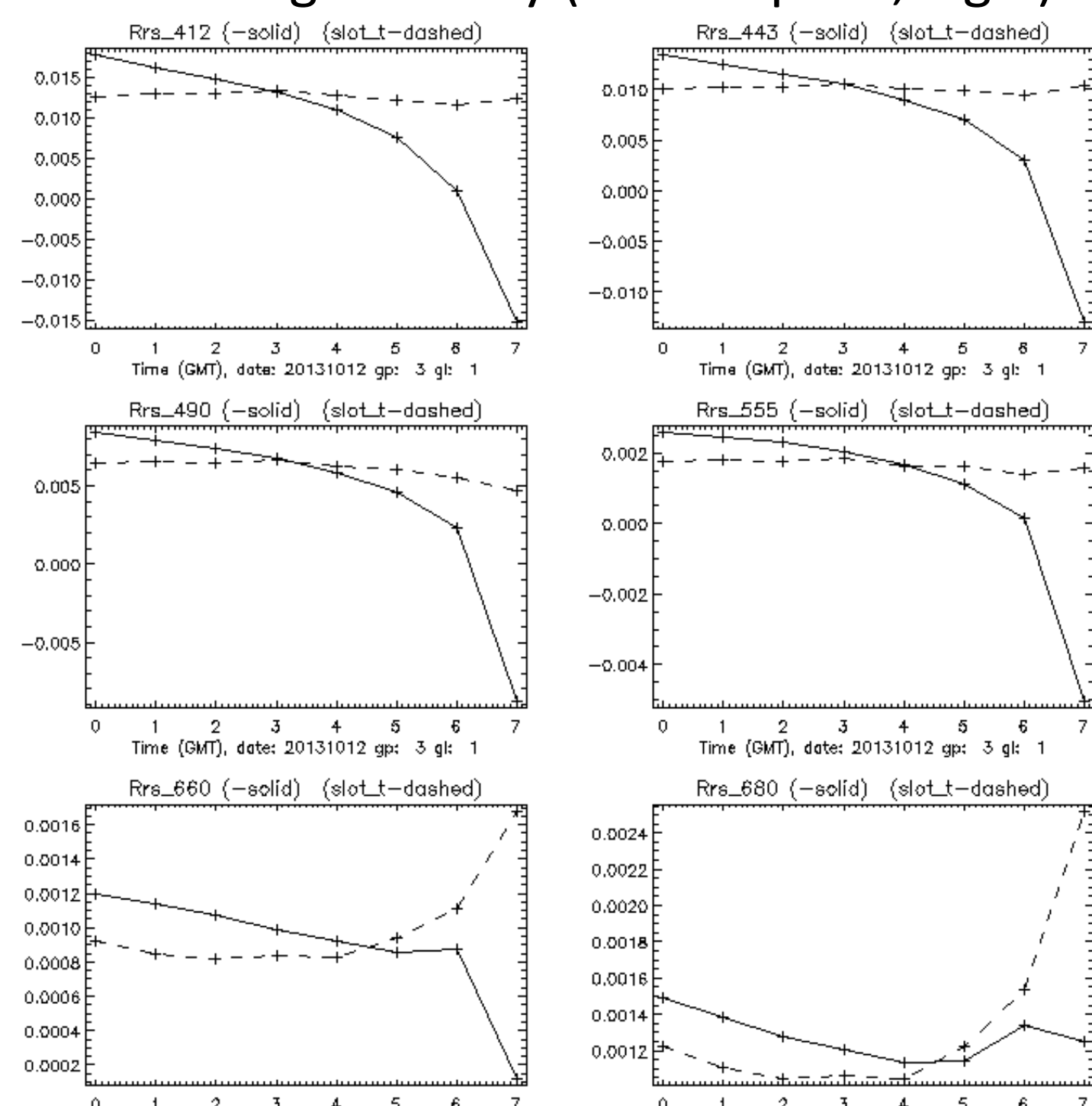
Figure 2. These 6 plots show the Rrs (remote-sensed reflectance) for the 6 GOCI visible bands as a function of time of day. Each point is the average of the non-cloud portion in the box shown in Fig 1. Rrs before (solid lines) and after (dashed) slot time use are plotted.
