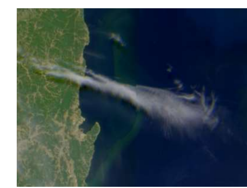
Figure 6. A close up view of the region A from Fig 5 showing a cirrus cloud moving off the Korean coast
