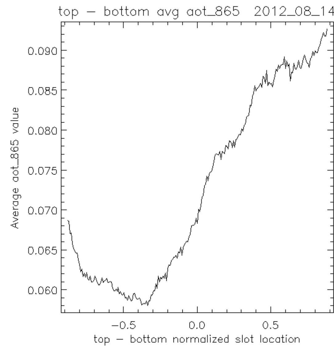
Figure 4. Average of all rows of aot_865, omitting row and column data < 0.12 units from the edge (15 pixels) to avoid edge effects (lack of data and data from scene bottom only due to slot stitching).
