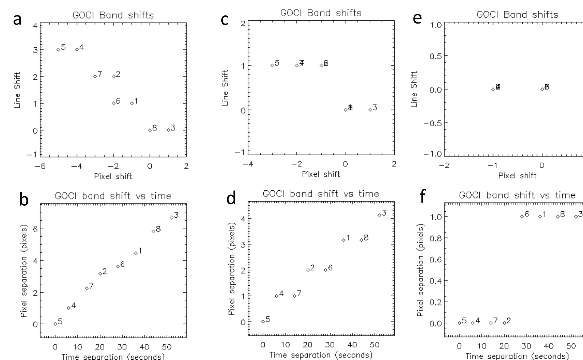
Figure 8. a, c, and e: Cloud shift in pixel and line relative to band 8 derived at points A, B, and C for the scene in Fig 5. Plots b, d, and f are the displacement of the cloud from band 5 (first acquired band) versus time. Bands are labeled with their band number. The shift at point A (plot b) indicates a wind speed of 127 kt, which is close to what was reported in the 250 mb upper air analysis. Point B had lower winds while point C, a group of cumulus clouds, had only a 1 pixel shift. Even so, the shift as a function of time remains monotonic (plot f).
