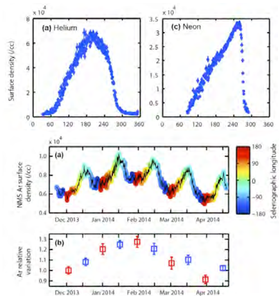
Fig. 2. (top) LADEE NMS results for ^4\text{He} and ^{20}\text{Ne} . Horizontal axis is solar longitude, with 0 at noon, 90 at sunset, 180 at midnight and 270 dawn. (bottom) Time variations in ^{40}\text{Ar} over the LADEE mission. Argon density maximizes over the western maria. From [7].
