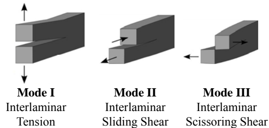
Figure 15. Fracture modes.
