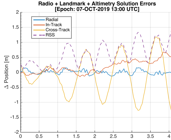
Figure 11. Position errors of the radio, landmark, and altimetric range trajectory solution with respect to the nominal “truth” trajectory in Radial, In-Track, and Cross-Track coordinates.
