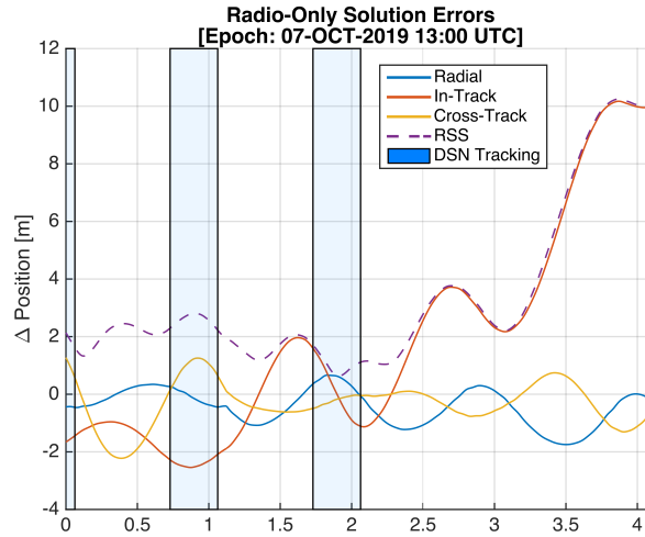
Figure 5. Position errors of the a radio-only trajectory solution with respect to the nominal “truth” trajectory in Radial, In-Track, and Cross-Track coordinates. Periods of DSN radiometric tracking (range and Doppler) used in the solution are shown in blue.
