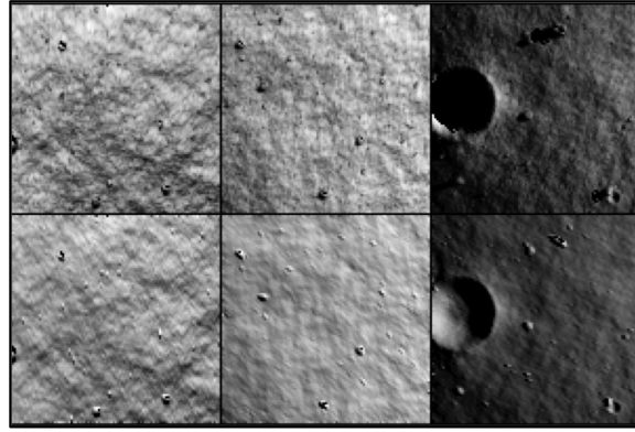
Figure 6. Extracted (top row) and predicted (bottom row) brightness for three maplets in the simulated image N623803681F1 (Epoch: October 8th, 2019 at 10:46:53 pm UTC).
