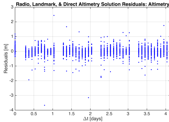
Figure 10. Post-fit altimetric range residuals for the radio, landmark, and altimetry data OD solution.
