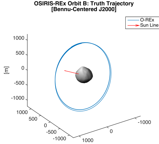
Figure 1. Nominal Orbit B trajectory in the Bennu-centered J2000 frame.
