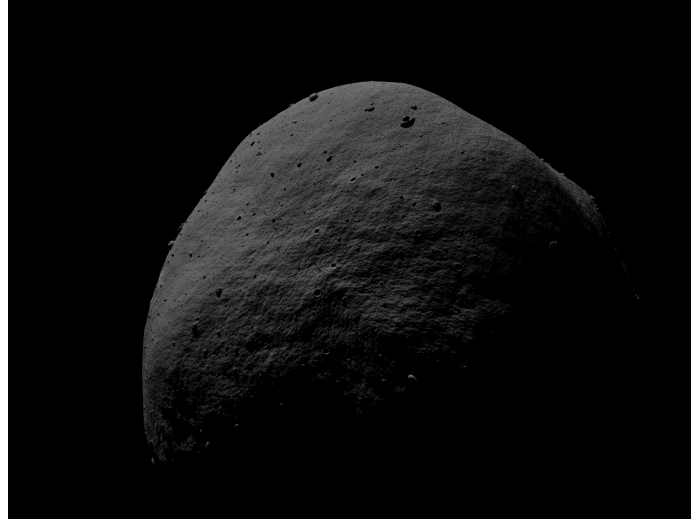
Figure 2. Simulated NavCam image using the simulated spacecraft and Bennu geometry from October 5th, 2019 at 2PM.
