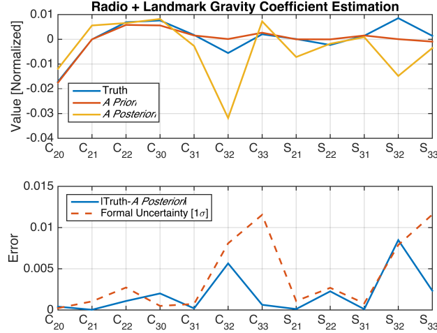
Figure 9. Truth, A Priori , and A Posteriori values for Bennu gravity coefficients (top) and associated errors and formal uncertainties (bottom) up to degree and order 3.
