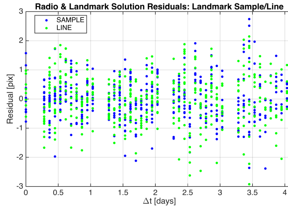
Figure 7. Post-fit landmark OpNav residuals for the radio plus landmark data OD solution.
