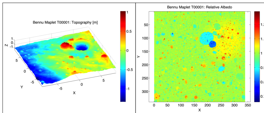
Figure 3. Local topography (left) and relative albedo (right) information for Bennu maplet T00001 (134.5 degrees longitude, 36.3 degrees latitude).
