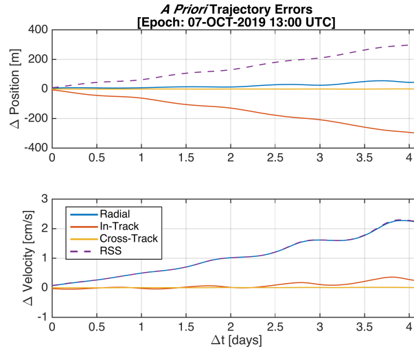
Figure 4. Position (top) and velocity (bottom) errors of the a priori trajectory with respect to the “truth” trajectory in Radial, In-Track, and Cross-Track coordinates.
