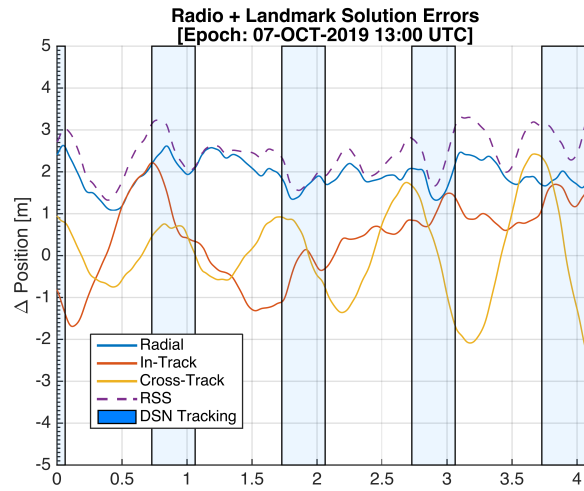
Figure 8. Position errors of the radio plus landmark trajectory solution with respect to the nominal “truth” trajectory in Radial, In-Track, and Cross-Track coordinates.
