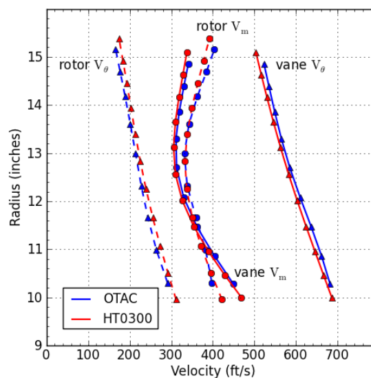
Figure 8 Comparison between OTAC and HT0300 calculated velocity components for the fourth stage of a five-stage LPT
