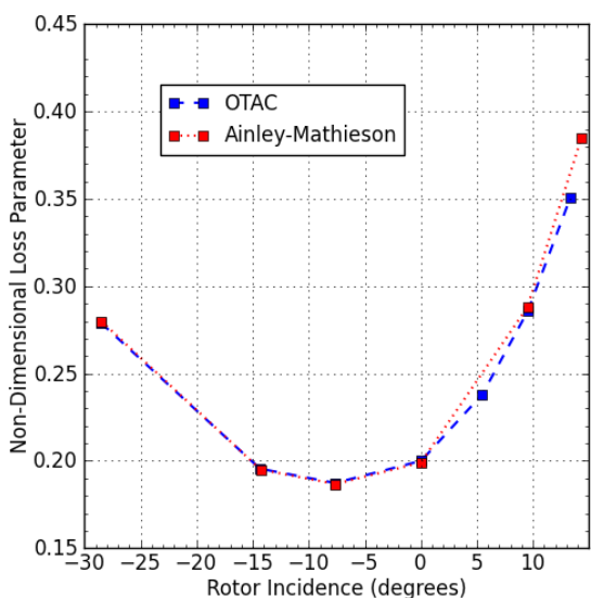
Figure 6 Comparison between OTAC and Ainley-Mathieson loss models as a function of rotor incidence
