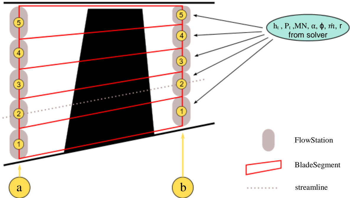
Figure 2 Objects used in the BladeRow assembly
