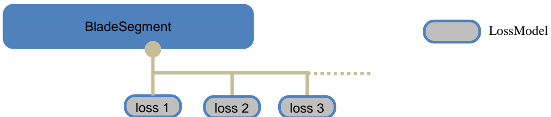
Figure 3 Schematic of a BladeSegment with attached losses; each LossModel object encapsulates a specific loss correlation and returns a value for loss parameter
