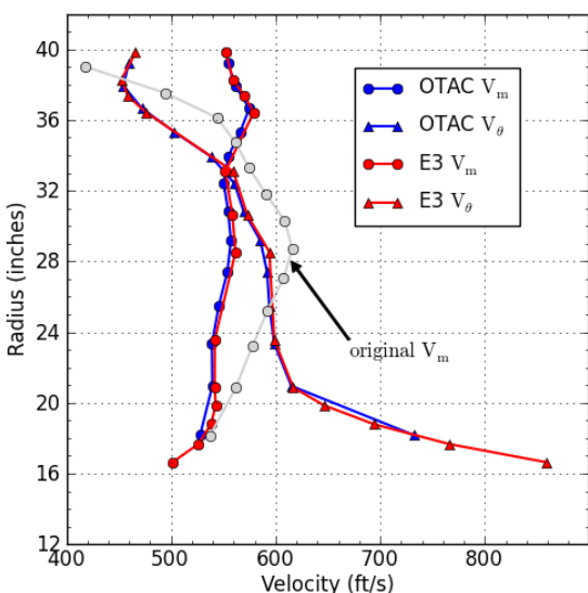
Figure 4 Comparison between OTAC and E 3 report values of velocity components for a single fan rotor
