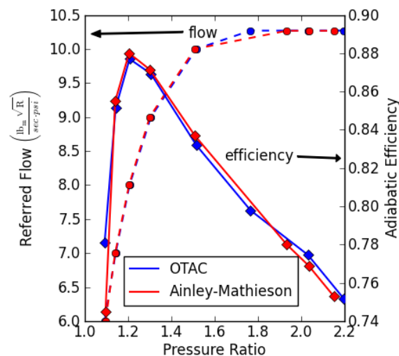
Figure 7 Comparison between OTAC and Ainley-Mathieson mass flow and efficiency characteristics for a single-stage turbine meanline calculation
