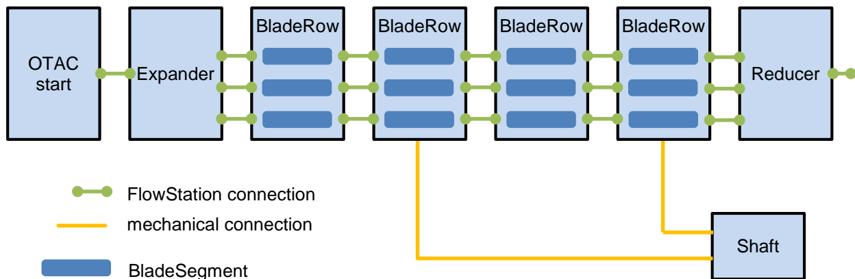
Figure 1 Object layout for a 2-stage, 3-stream OTAC example model
