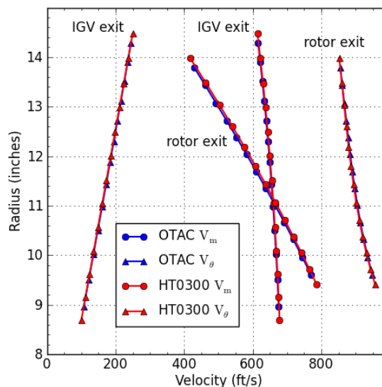
Figure 5 Comparison between OTAC and HT0300 calculated values of velocity components for an IGV followed by a rotor
