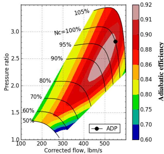
Figure 10 Performance of a 2-stage fan calculated by OTAC using 9 streamlines; the aerodynamic design point (ADP) is also shown
