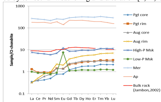
Figure 3: CI-chondrite normalized REE-patterns of zoned clinopyroxenes, plagioclases, phosphates and bulk composition in NWA 856.
