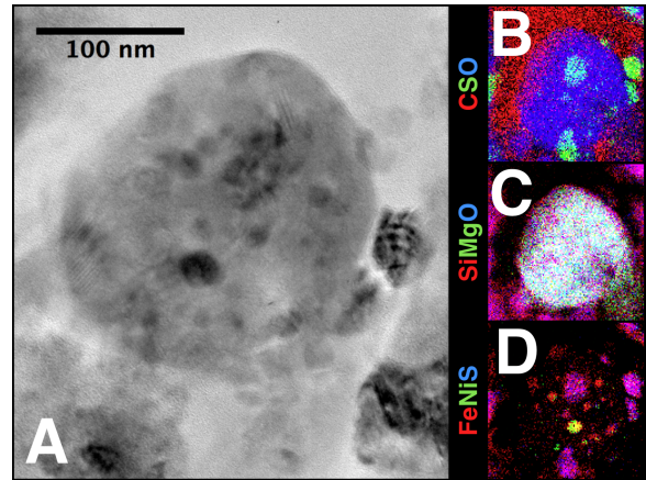
Figure 1: (A) TEM brightfield image of Daisy showing a rounded morphology and embedded crystals. The scale bar is 100 nm. (B) EDS map with C (red), S (green), O (blue) showing that the object contains sulfides and is surrounded by sulfides and epoxy. (C) EDS map with Si (red), Mg (green), O (blue) showing the object is Mg rich relative to surrounding silicate. (D) EDS map with Fe (red), Ni (green), S (blue) showing Ni-rich metal, Ni-poor metal and sulfide.
