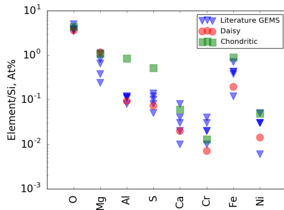
Figure 2: Plot of the elemental composition of a suite of GEMS in anhydrous IDPs normalized to Si in At% from Bradley and Ireland[11] compared to Daisy. Chondritic composition is also plotted.
