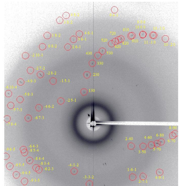
Fig. 3. XRD pattern of the cordierite-like phase in Al-rich chondrule in Y-82094 with indices (yellow numbers next to red circles) using the indialite crystal structure. Successful indexing by the indialite structure reveals that this phase is indialite rather than cordierite.
