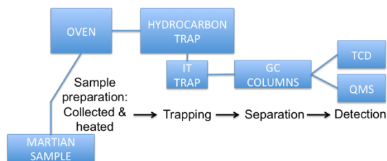
Figure 1: simplified analytical channel from sample collection to the detection and identification of the organic molecules.
