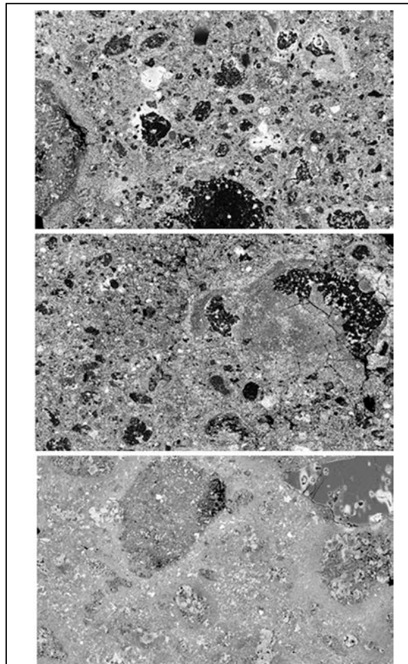
Figure 1. BSE Images of JW lithologies. Degree of heating and brecciation increases downward. 1 mm across.
