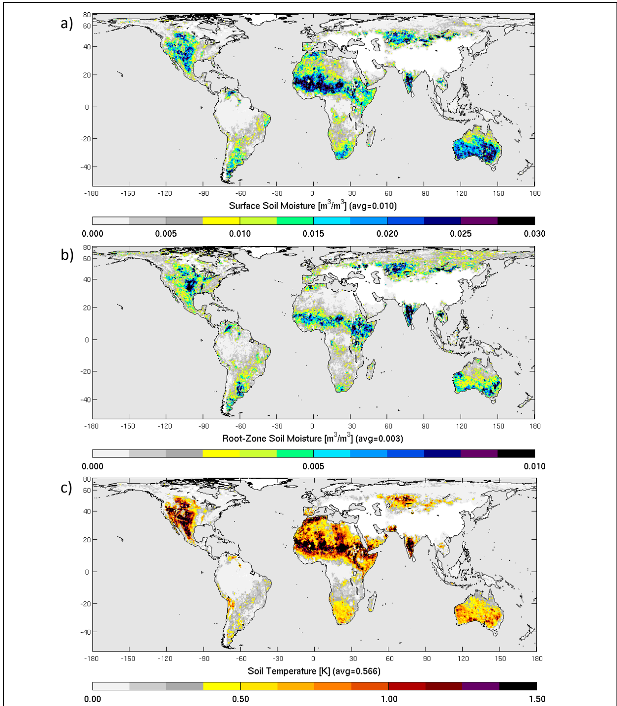
Figure 21. Same as Figure 20 but for time series standard deviation of the increments. Note the difference in colorscale for (a) and (b).
