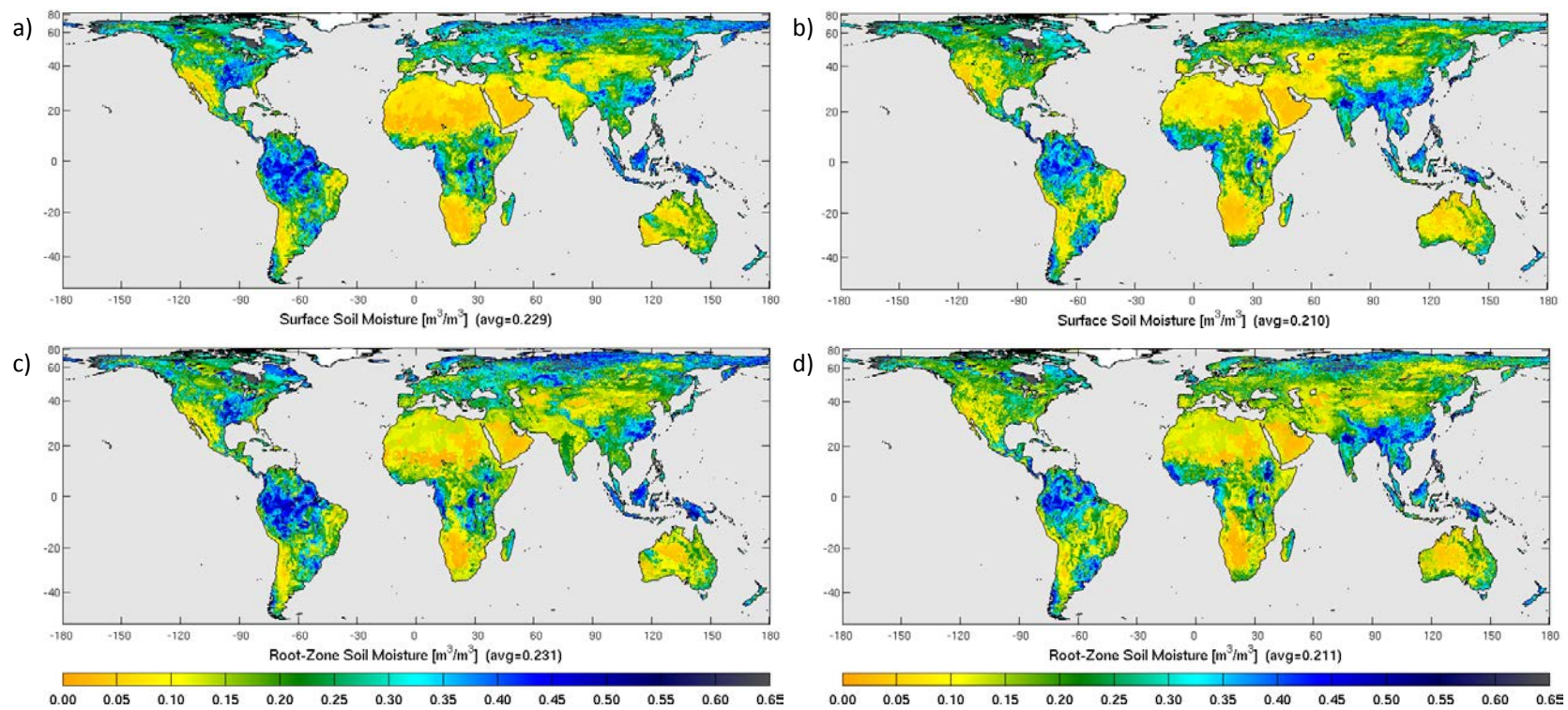
Figure 4. Snapshots of L4_SM (a,b) surface and (c,d) root zone soil moisture for (a,c) 1 June 2015, 0z, and (b,d) 1 September 2015, 0z.
