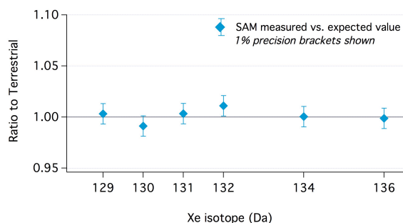
Figure 1: Static mode performance of the SAM QMS demonstrates the 1-2% precision in isotopic measurements achieved in short integration times. The entire set of measurements that generated the ratio plot in the bottom frame was acquired in 30s [8].
