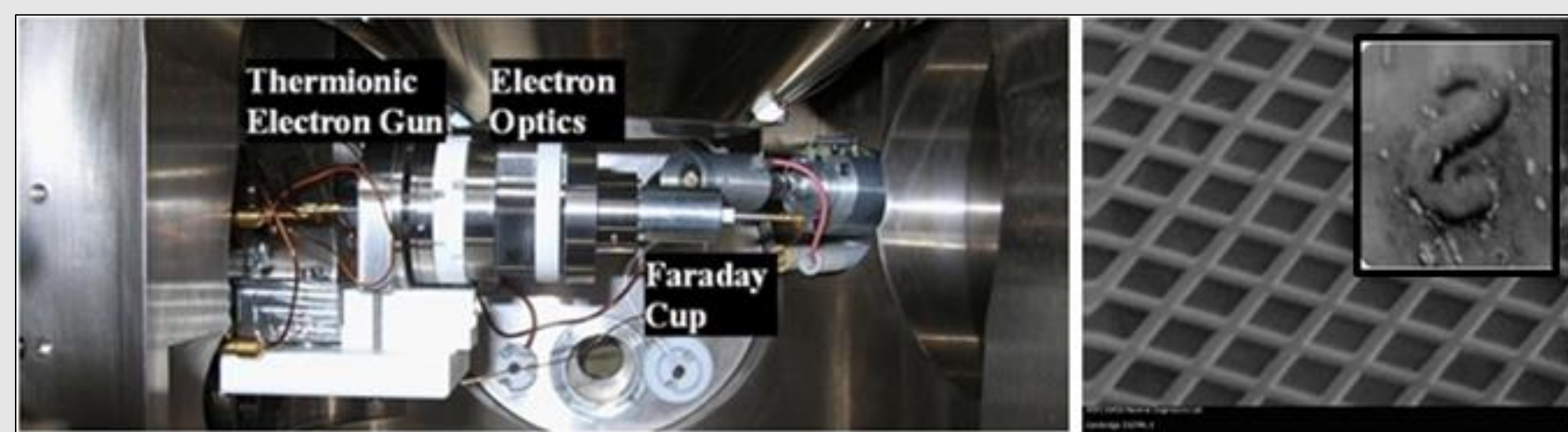
Figure 1: (Left) Lunar Miniaturized Scanning Electron Microscope attached to a commercial-off-the-shelf (COTS) electron gun. A Faraday cup was attached to measure beam current, which was later replaced with a scanning coil assembly for imaging. (Right) The instrument's images of a copper grid standard and the letter "S" on a penny. (Credit: NASA/J. Gaskin)
