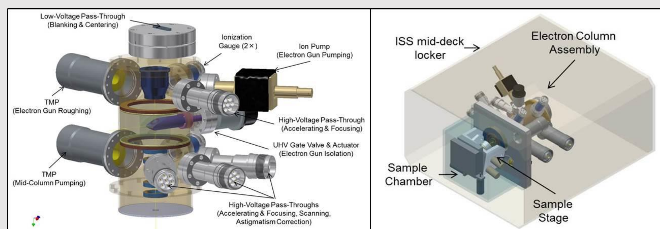
Figure 2: (Left) ISS miniaturized SEM electron column layout. This layout includes the electron column, pumps, vacuum gauges, and high voltage pass-throughs. The main assembly is slightly larger than a 12oz soda can. (Right) Diagram on the electron column assembly inside of a mid-deck locker on the ISS as shown. A sample chamber has been designed to allow for manual sample insertion. (Credit: Creare/R. Klein-Schoder and reproduced with permission)
