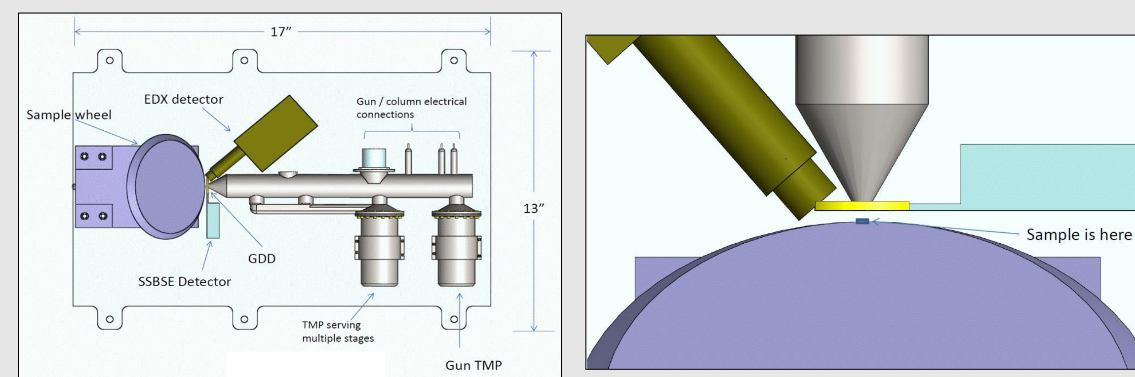
Figure 3: (Left) Preliminary feasibility concept for the MVP-SEM. The current concept has roughly a 17" x 13" footprint. (Right) Zoomed-in drawing of the sample region. The detectors shown are a combination of COTS and custom and are meant to allow for conceptual visualization. This design will change as the instrument requirements solidify and the development progresses. (Credit: JPL-Caltech/E. Neidholdt)
