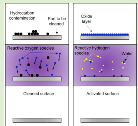
FIGURE 2 Illustration of the effects of plasma cleaning with oxygen (left) and hydrogen (right)
