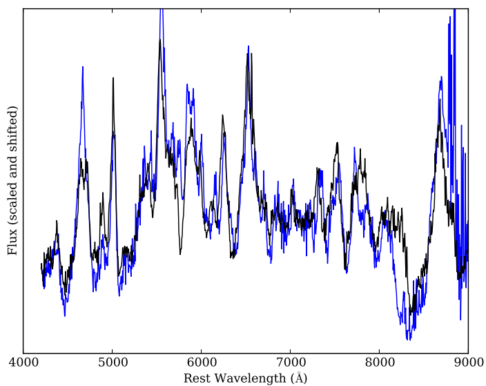
Fig. 20.— Comparison between PTF 09eyi (blue, +55 days) and SN 2002cx (black, +56 days). The former has had galaxy light subtracted via Superfit, and the fiducial redshift of 0.06 was used to align spectra.
