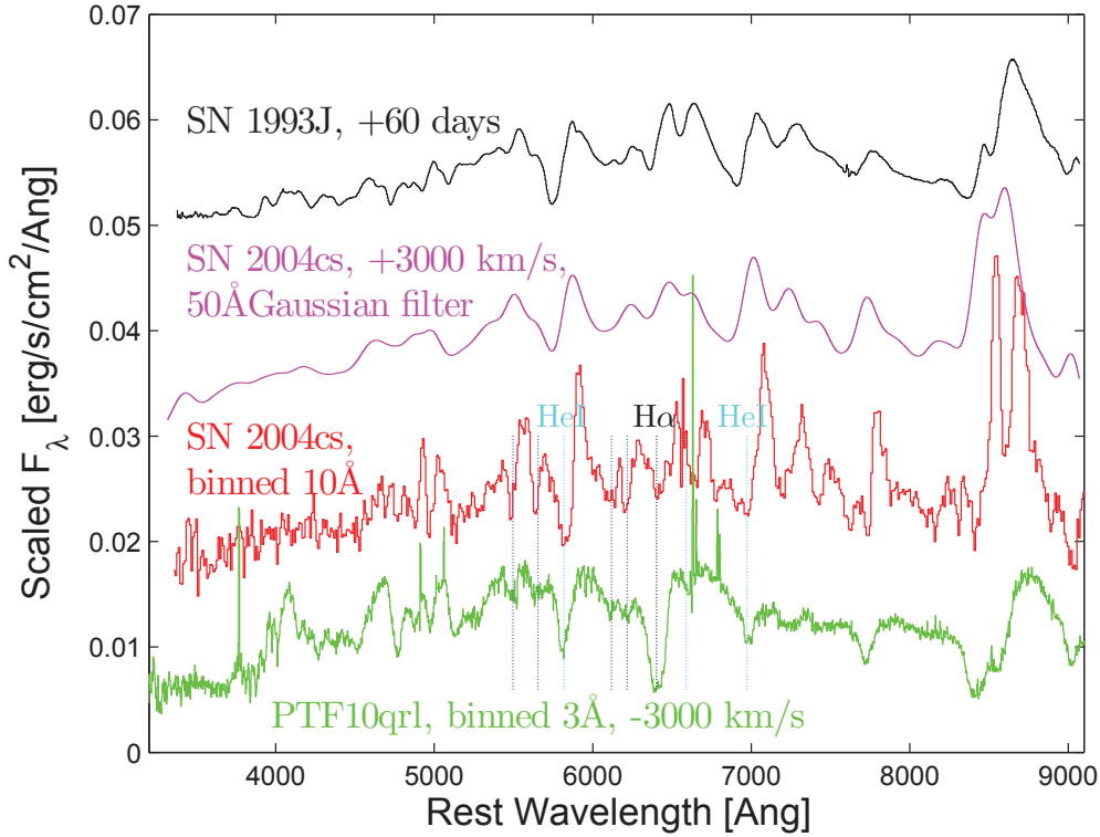
Fig. 16.— Comparison of spectra of SN 2004cs (red) and PTF 10qrl (green, a low-velocity SN IIB) showing excellent alignment of features. Absorption lines of hydrogen ( H\alpha , black) and He I (5876 Å and 7065 Å, cyan) are clearly identified, and additional nearby features (blue) also perfectly align. A broadened and blueshifted version of the SN 2004cs spectrum (magenta) also displays a strong similarity to a spectrum of the prototypical Type IIB SN 1993J (black).
