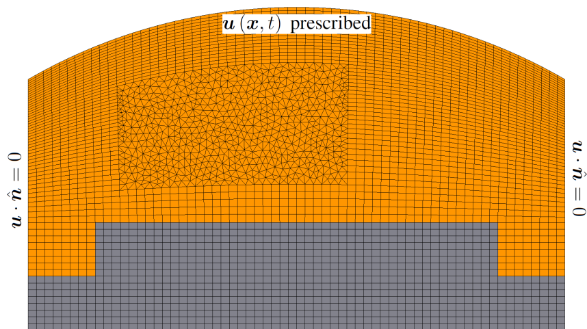
Figure 3. Canonical arcjet iso-q geometry for mesh motion demonstration case.
