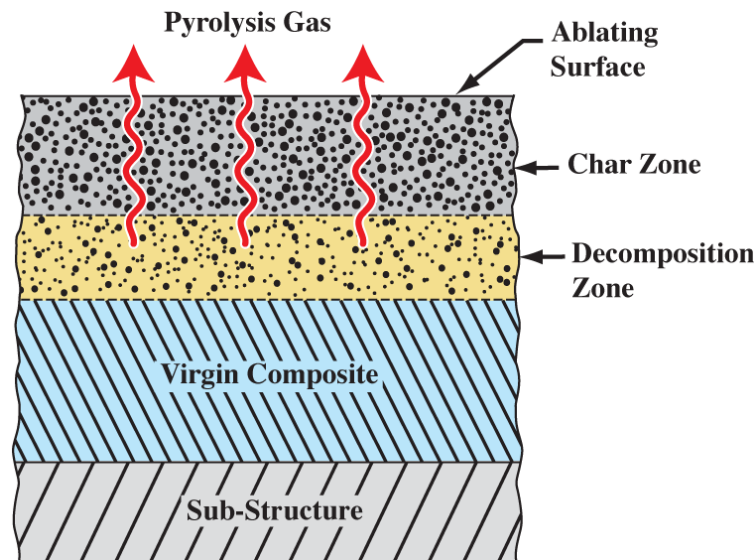
Figure 1. In-depth schematic of a charring (pyrolyzing) ablator.
