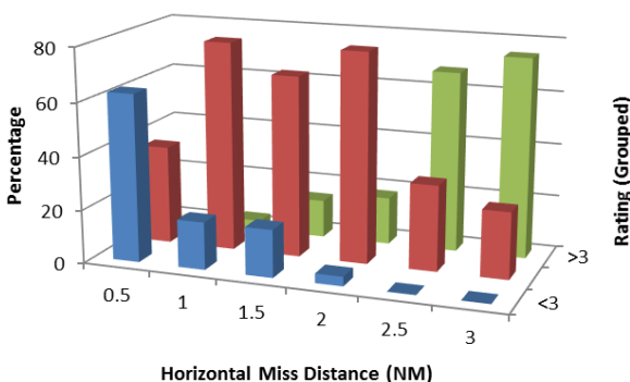
Figure 4. Subject controllers' ratings for HMD spacing parameters for the overtake encounter geometry.
