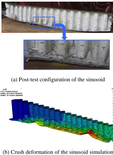
Figure 28. Post-test and simulation results for the sinusoid
