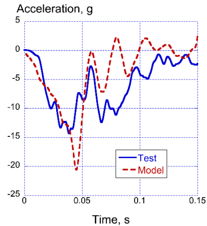
(a) Forward acceleration
