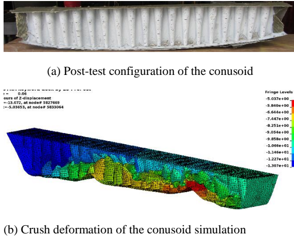
Figure 27. Post-test and simulation results for the conusoid
