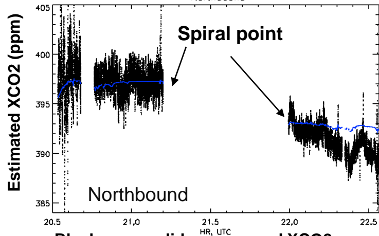
Black curves: lidar measured XCO2 Blue curves: in-situ derived XCO2
