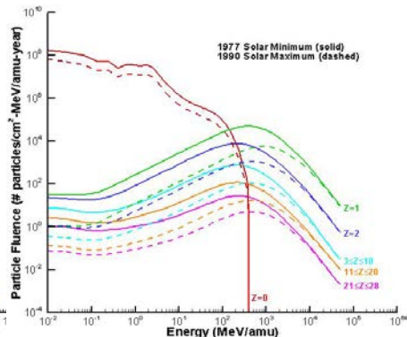
Lunar surface environment due to GCR
