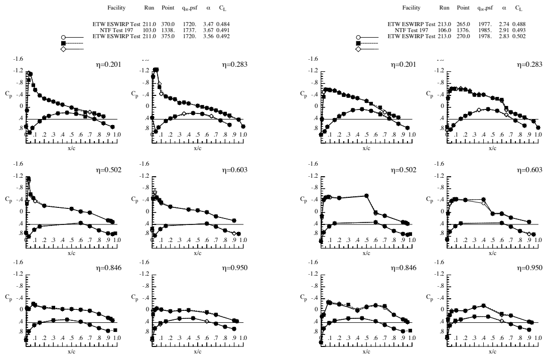
Figure 13: Surface pressures, Re_c = 19.8 \times 10^6 , high q_\infty , Mach=0.7 (left) and Mach=0.85 (right).
