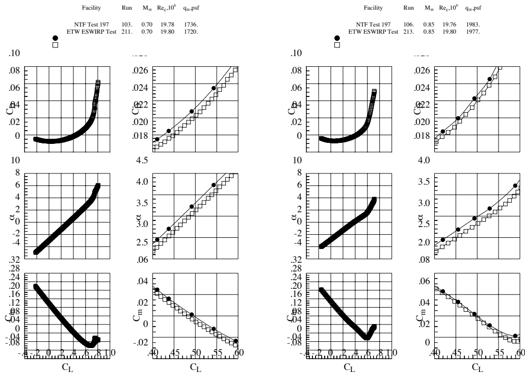
Figure 9: Lift, drag and pitching moment coefficients, Re_c = 19.8 \times 10^6 , high q_\infty , Mach=0.7 (left) and Mach=0.85 (right).
