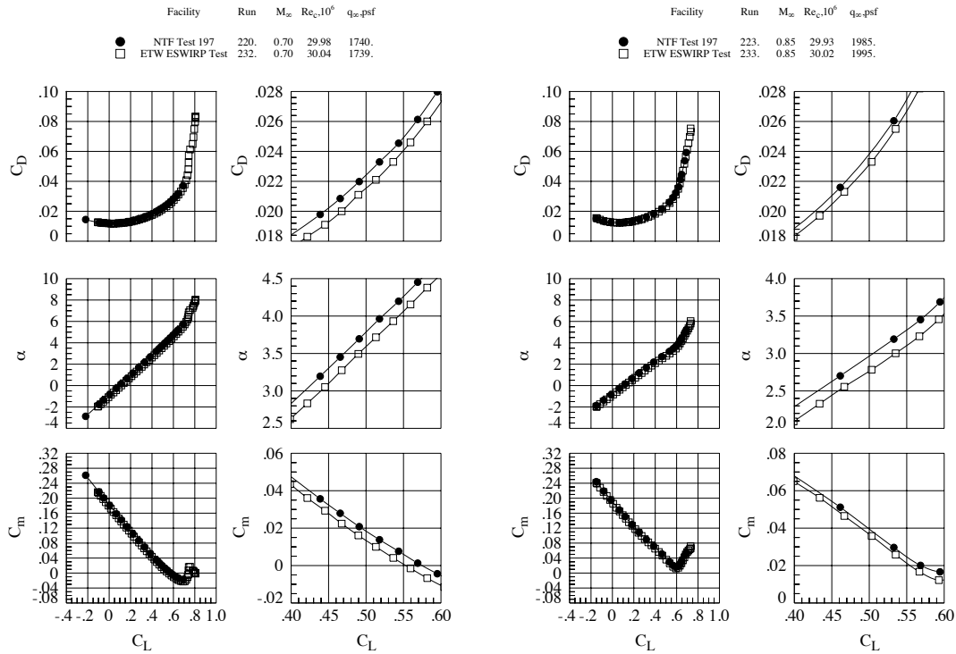
Figure 10: Lift, drag and pitching moment coefficients, Re_c = 30 \times 10^6 , Mach=0.7 (left) and Mach=0.85 (right).
