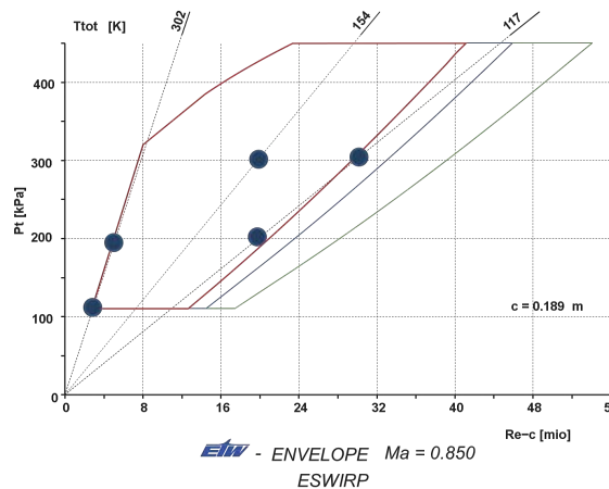
Figure 6: ETW test envelope at Mach = 0.85.
