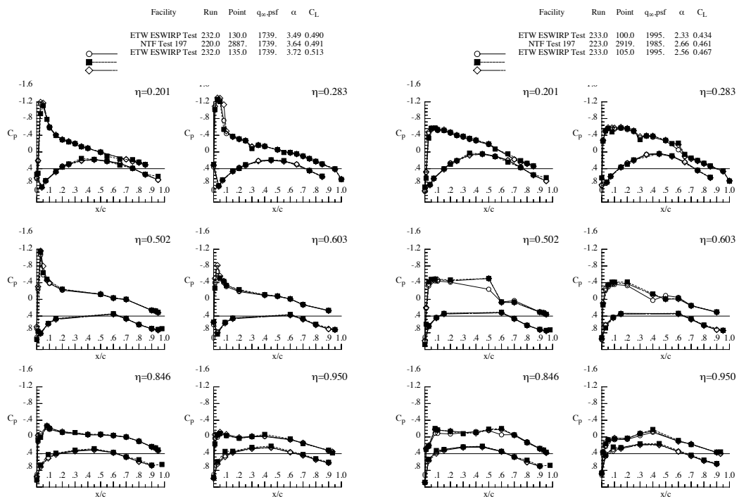
Figure 14: Surface pressures, Re_c = 30 \times 10^6 , high q_\infty , Mach=0.7 (left) and Mach=0.85 (right).
