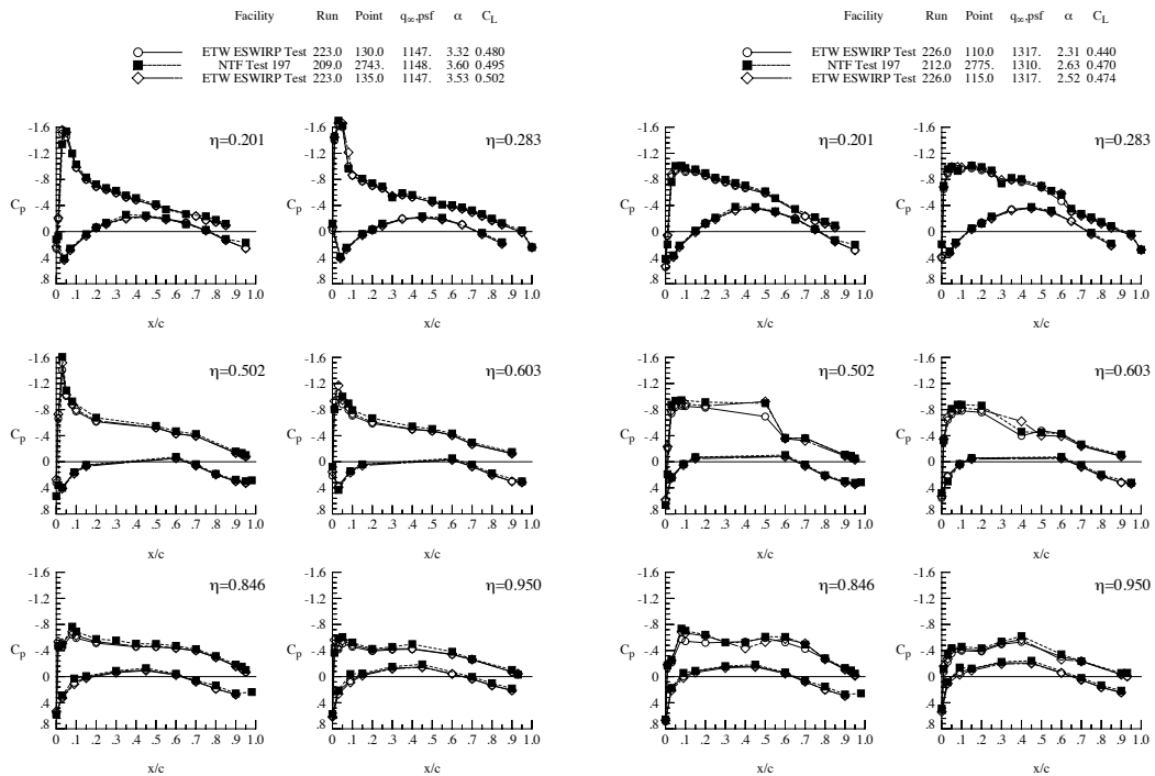
Figure 12: Surface pressures, Re_c=19.8 \times 10^6 , low q_\infty , Mach=0.7 (left) and Mach=0.85 (right).
