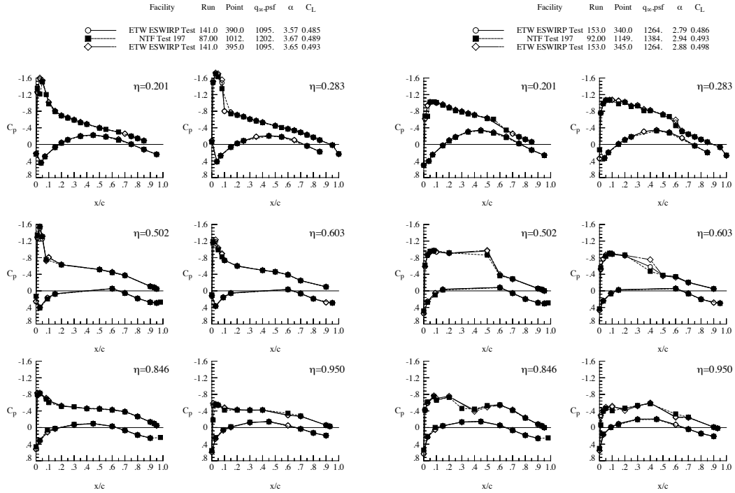
Figure 11: Surface pressures, Re_c=5 \times 10^6 , Mach=0.7 (left) and Mach=0.85 (right).
