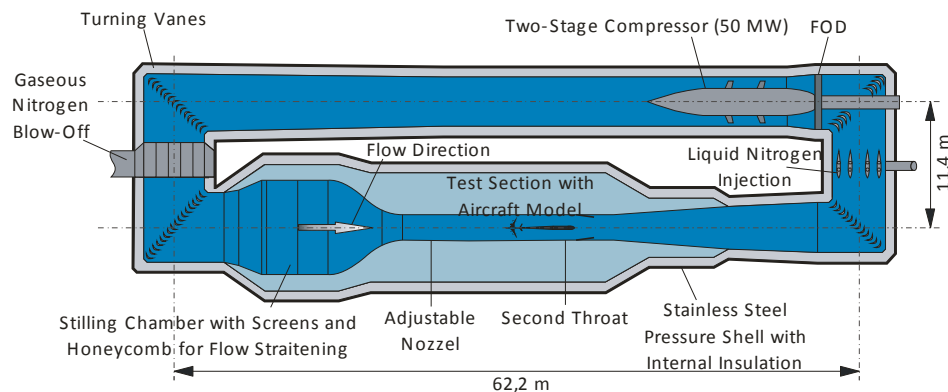
Figure 3: Sketch of the European Transonic Wind Tunnel aerodynamic circuit.
