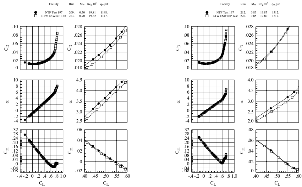
Figure 8: Lift, drag and pitching moment coefficients, Re_c = 19.8 \times 10^6 , low q_\infty , Mach=0.7 (left) and Mach=0.85 (right).
