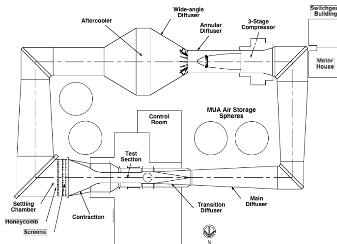
Figure 2: Sketch of the Ames 11-Foot Wind Tunnel.
