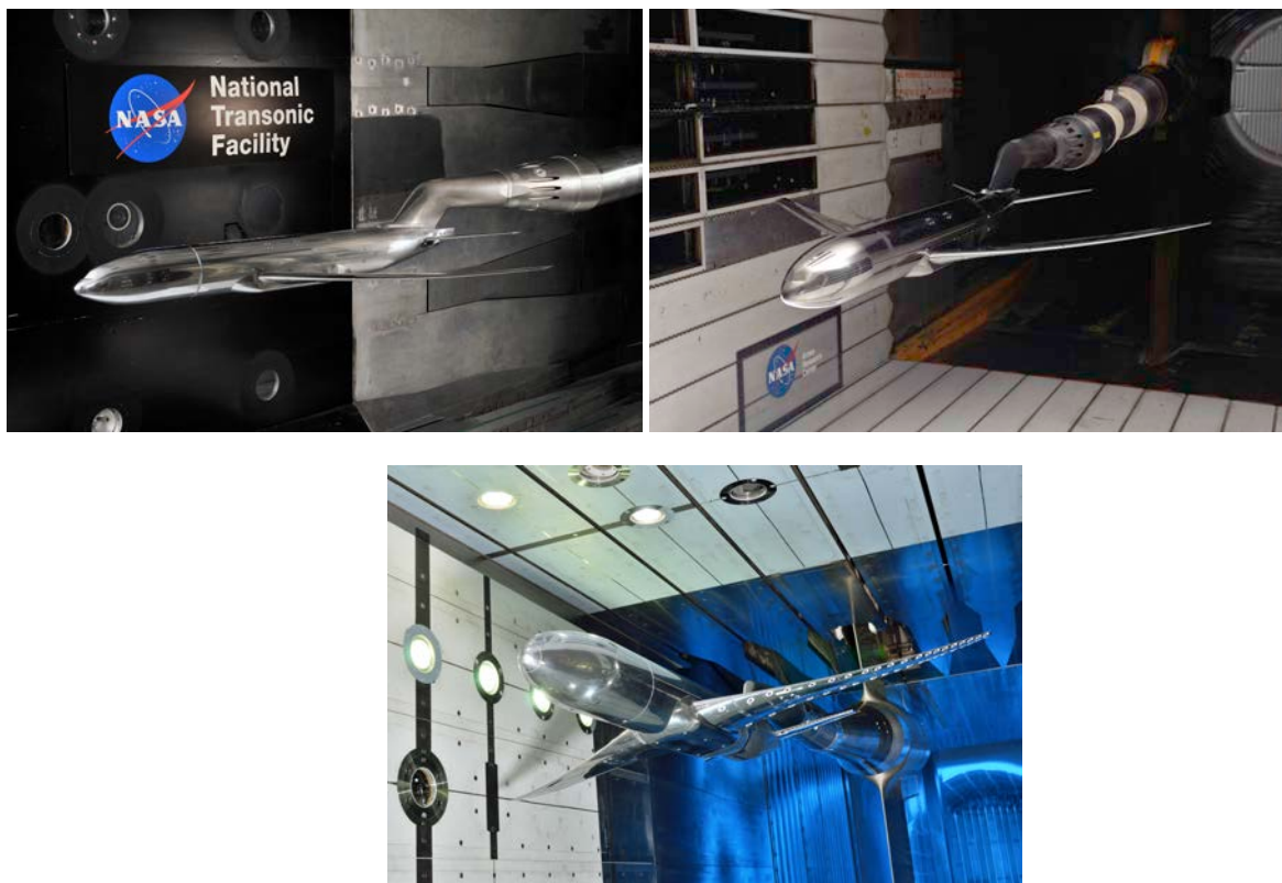
Figure 5: Photo of the Common Research Model in the National Transonic Facility (top left) and the Ames 11-ft Wind Tunnel (top right) and the European Transonic Wind Tunnel (bottom).
