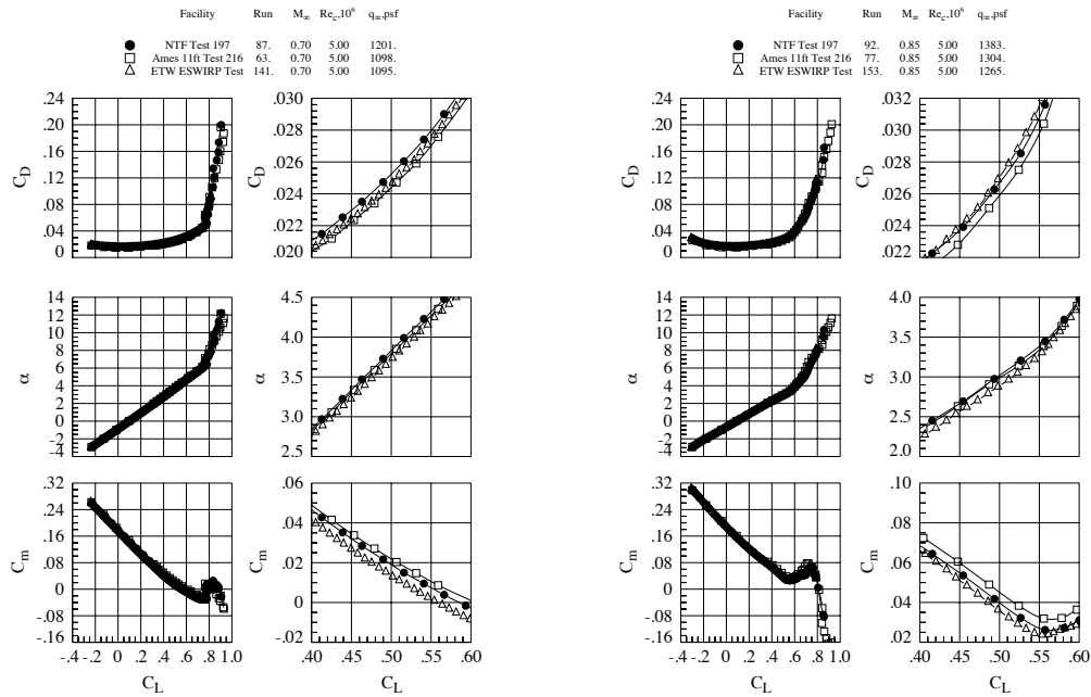
Figure 7: Lift, drag and pitching moment coefficients, Re_c = 5 \times 10^6 , Mach=0.7 (left) and Mach=0.85 (right).
