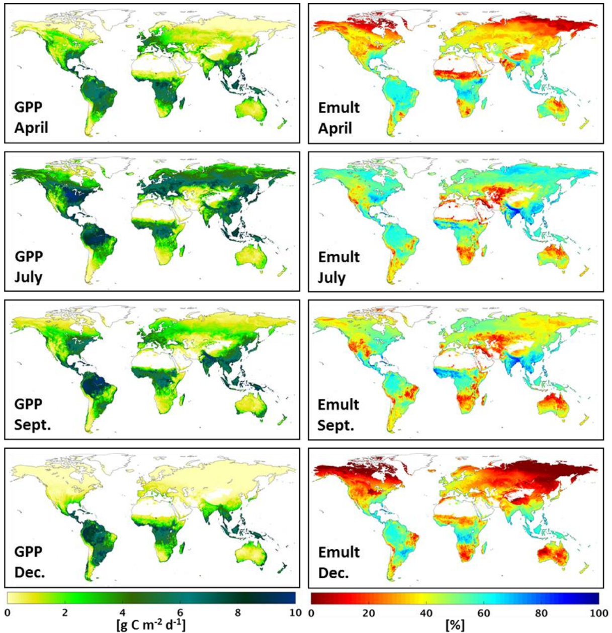
Figure 7.1. L4_C product monthly averages for April, July, September, and December 2015, showing vegetation gross primary production (GPP) and the GPP-based environmental constraint (Emult), which is the proportion (%) of estimated light use efficiency relative to a potential maximum rate ( LUE/LUE_{mx} ) defined for optimal (non-limiting) environmental conditions. The Emult metric is a dimensionless scalar ranging from 0 (fully constrained) to 100% (no constraint). White areas denote barren land, permanent ice, open water and other areas outside of the model domain.
