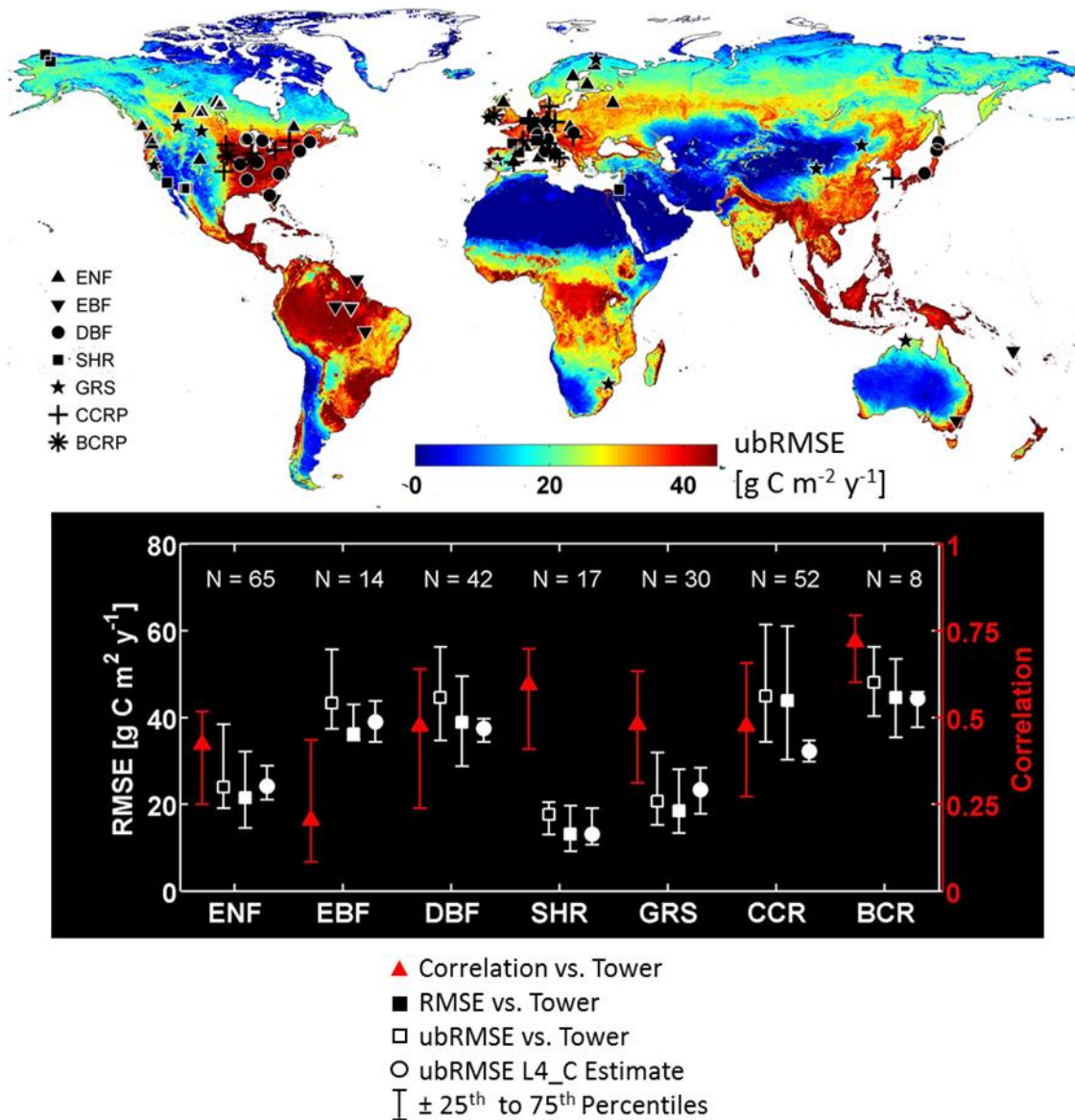
Figure 7.5. Estimated L4_C model and product performance for NEE in relation to in situ observations from 228 La Thuile tower sites representing the major global plant functional type (PFT) classes, including evergreen needleleaf forest (ENF), evergreen broadleaf forest (EBF), deciduous broadleaf forest (DBF), shrubland (SHR), grassland (GRS), cereal (C3) croplands (CCR) and broadleaf (C4) croplands (BCR). The tower sites are depicted in the L4_C model-estimated NEE ubRMSE (g C m -2 yr -1 ) map (top). The lower plot includes a summary of mean model and tower NEE correlations and RMSE differences within each PFT class, with associated 25 th and 75 th percentiles of spatial variability; the number (N) of La Thuile tower observation sites represented within each PFT class is denoted at the top of the plot. The estimated mean ubRMSE levels derived from the model sensitivity simulations (shown in upper map) for the tower pixel locations are also summarized within each PFT class in the plot.
