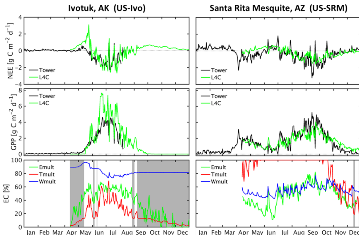
Figure 7.8. L4_C time series (April 13, 2015 – December 31, 2015) examples for tussock tundra (Ivotuk) and semi-arid shrubland (Santa Rita Mesquite) CVS tower sites. L4_C results shown for local tower PFT conditions (SHR for both locations with 85% and 17% of overlying 9-km L4_C grid cell coverage, respectively). Shaded regions indicate frozen conditions defined from the L4_C Frozen Area QA metric (Glassy et al. 2015).
