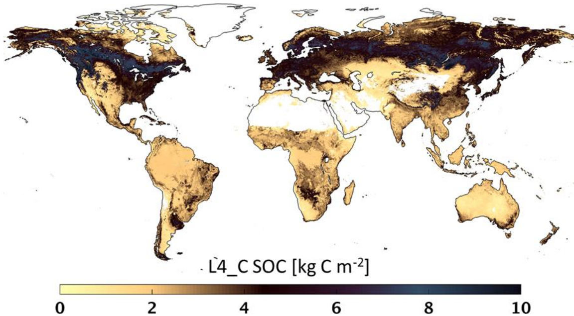
Figure 7.4. Estimated surface ( < 10 cm depth) soil organic carbon (SOC, \text{kg C m}^{-2} ) for April 15, 2015 from the SMAP L4_C operational record. The SOC estimates are derived at a 1-km spatial resolution during L4_C processing and posted to a 9-km resolution spatial grid. White areas denote barren land, permanent ice, open water and other areas outside of the model domain.
