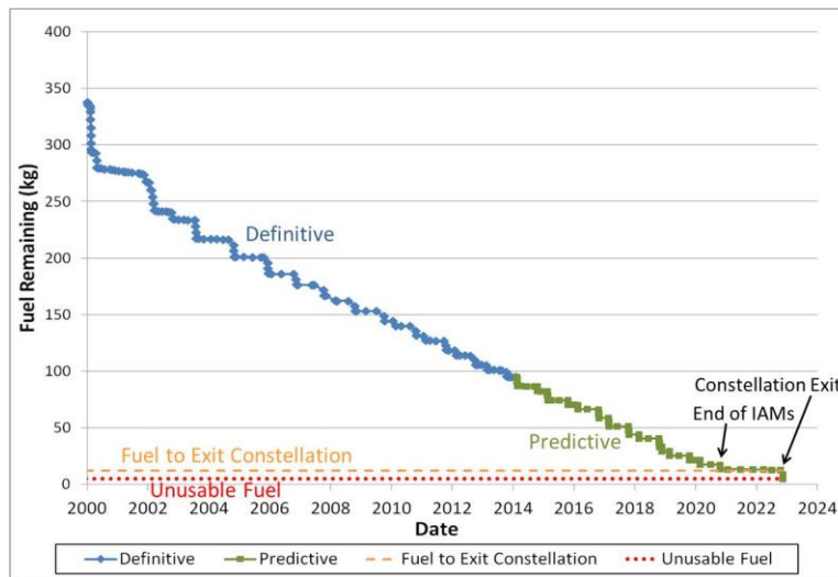
Figure 8. Terra Fuel Usage under Option 2 (Actual and Predicted) for 2000 - 2022
