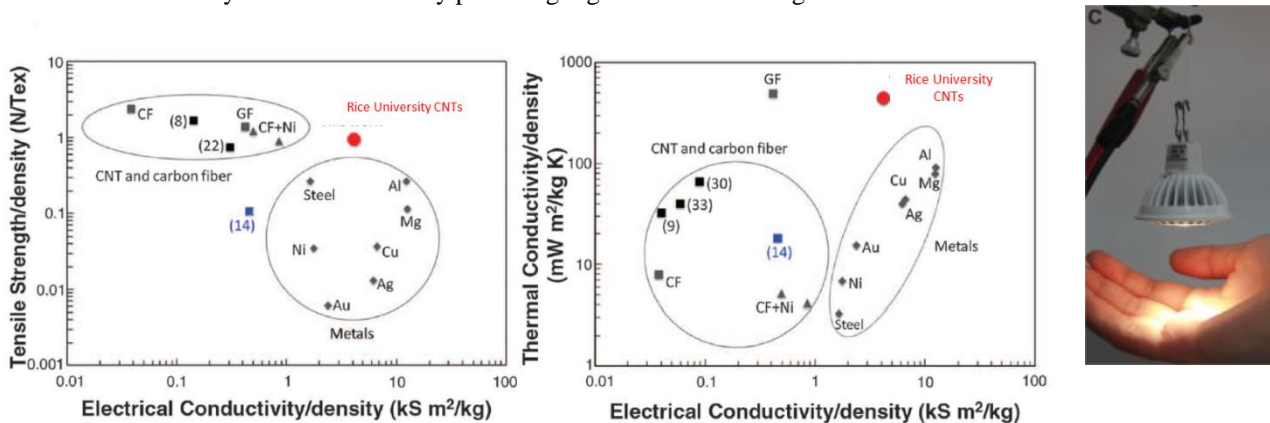
Figure 4. (Left and Middle) Ashby plots showing the CNT fiber properties developed by Rice University. (Right) Demonstration of the mechanical strength of CNT fiber developed by Rice University 12 .
