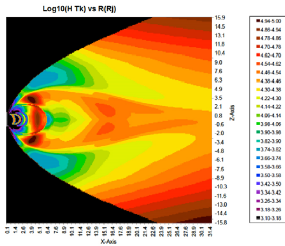
Figure 16. Meridional contour plots of the three proton Kappa parameters (Kappa value, density, and temperature) as fit to the DG2 plasma model and the new high energy proton model. The energy range of applicability is from \sim 1 keV up to \sim 600 keV.
