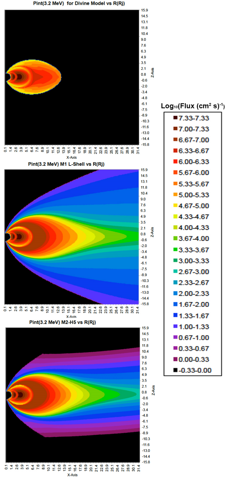
Figure 6. Comparison of the log 10 of the proton integral flux (E>3.2 MeV) between (top) the original (DG1) Divine-Garrett model; (middle) the new (DG2) GIRE2 model assuming that the equatorial fluxes are constant along a given L-shell; and the new GIRE2 model assuming that the fluxes fall off with a scale height of 5 R J beyond L>17 (see text).
