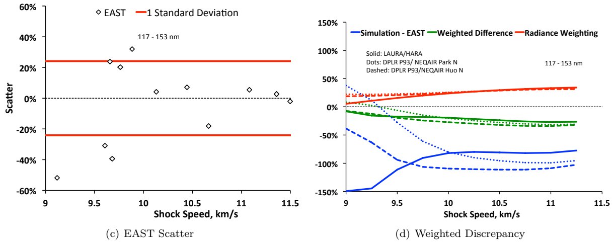
Figure 4. Comparison of EAST, NEQAIR and HARA for the 117 to 153 nm spectral region using the absolute non-equilibrium metric.
