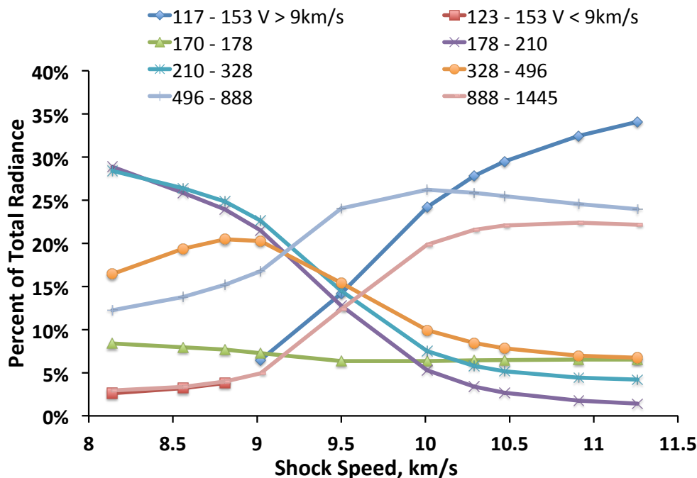
Figure 3. Percentage of radiance emitted from various spectral regions as calculated by HARA.
