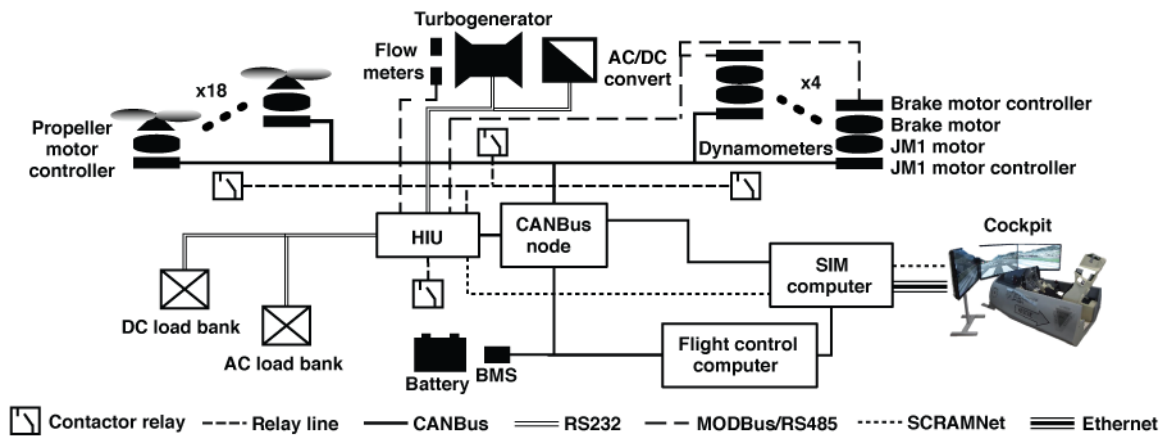
Figure 1. HEIST Testbed communication bus architecture.
