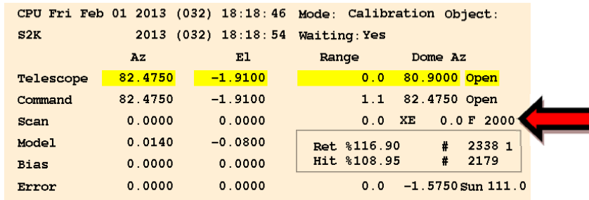
Figure 6-13: Ratgui main window showing that the SLR laser is firing at 2 kHz
